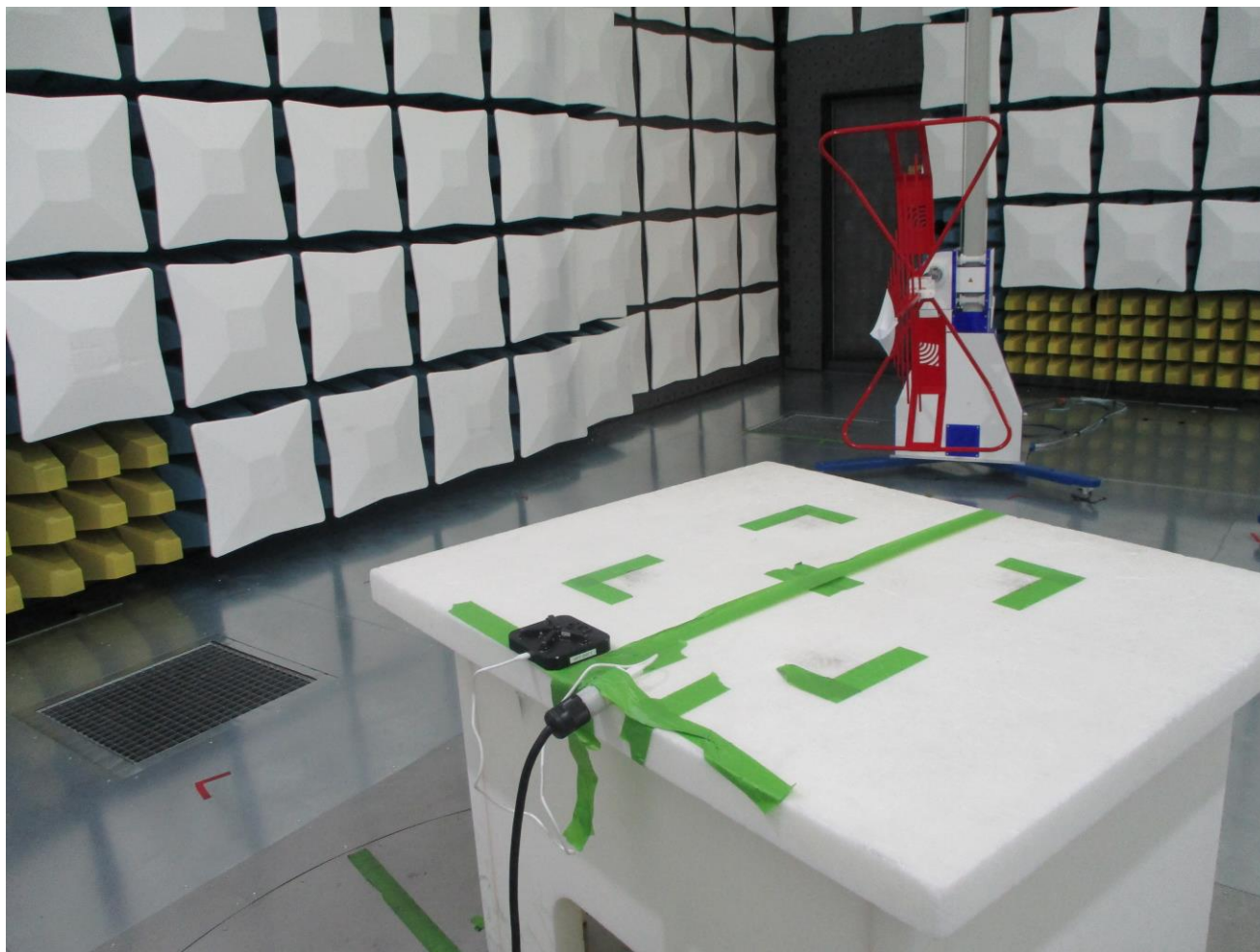
Figure 6: 30MHz-1GHz Test Setup (Rear View)
