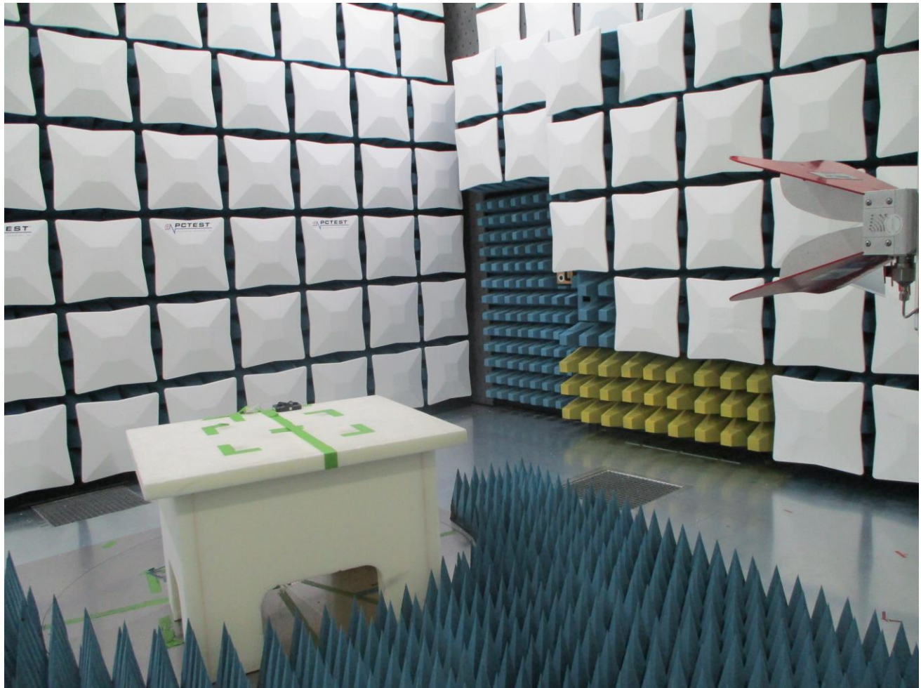
Figure 3: Above 1GHz Test Setup (Front View)
