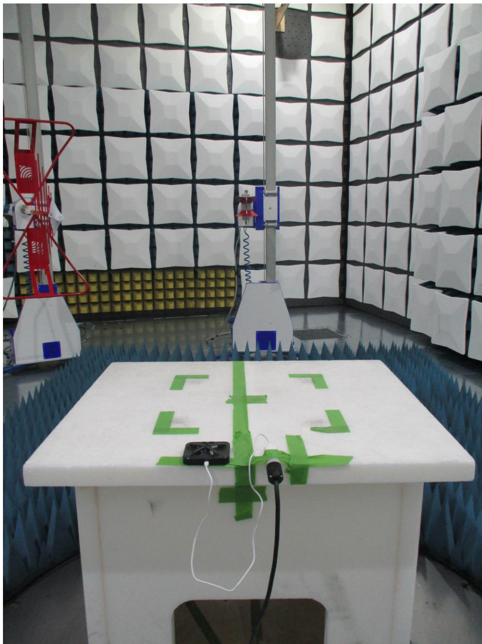
Figure 4: Above 1GHz Test Setup (Rear View)
