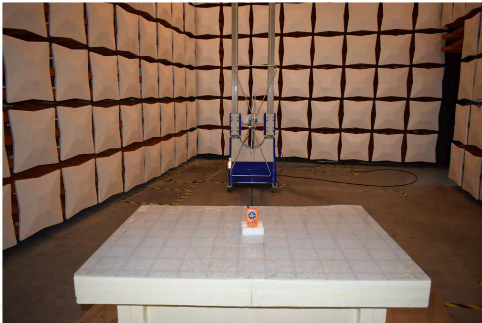
TX 30MHz~1GHz
