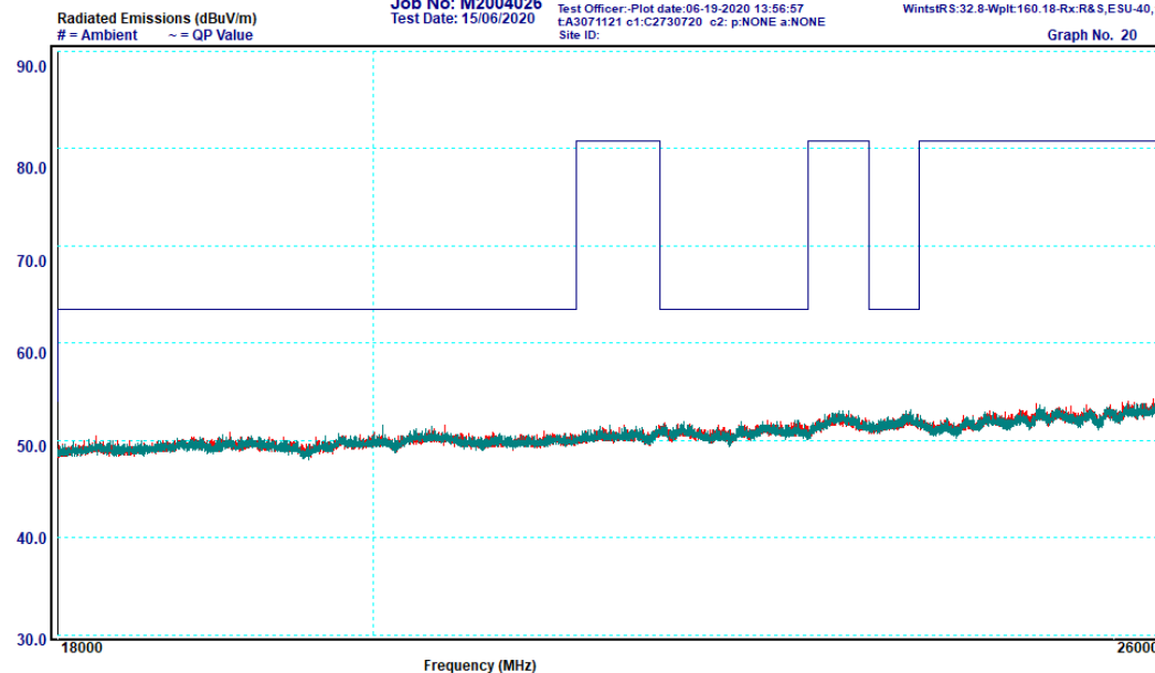
Graph 6-23: Transmitter Spurious Emissions, 18 – 26 GHz, 2402 MHz, Average
