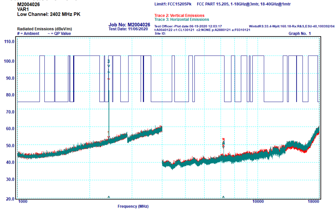
Graph 6-14: Transmitter Spurious Emissions, 1 – 18 GHz, Low Channel 2402 MHz, Peak
