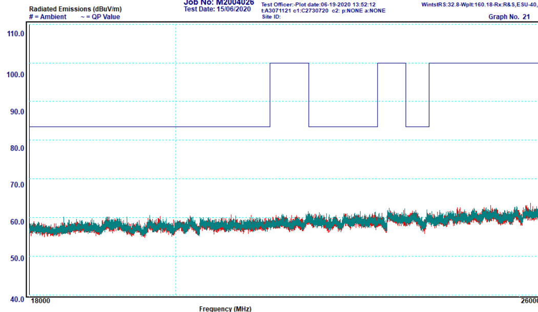
Graph 6-21: Transmitter Spurious Emissions, 18 – 26 GHz, 2440 MHz, Peak
