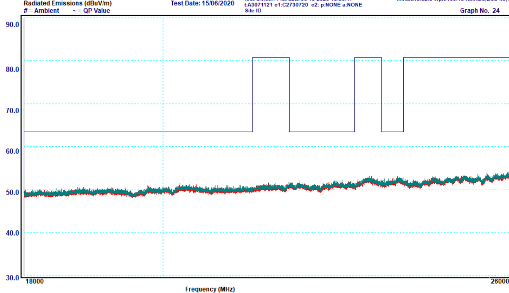
Graph 6-25: Transmitter Spurious Emissions, 18 – 26 GHz, 2480 MHz, Average
