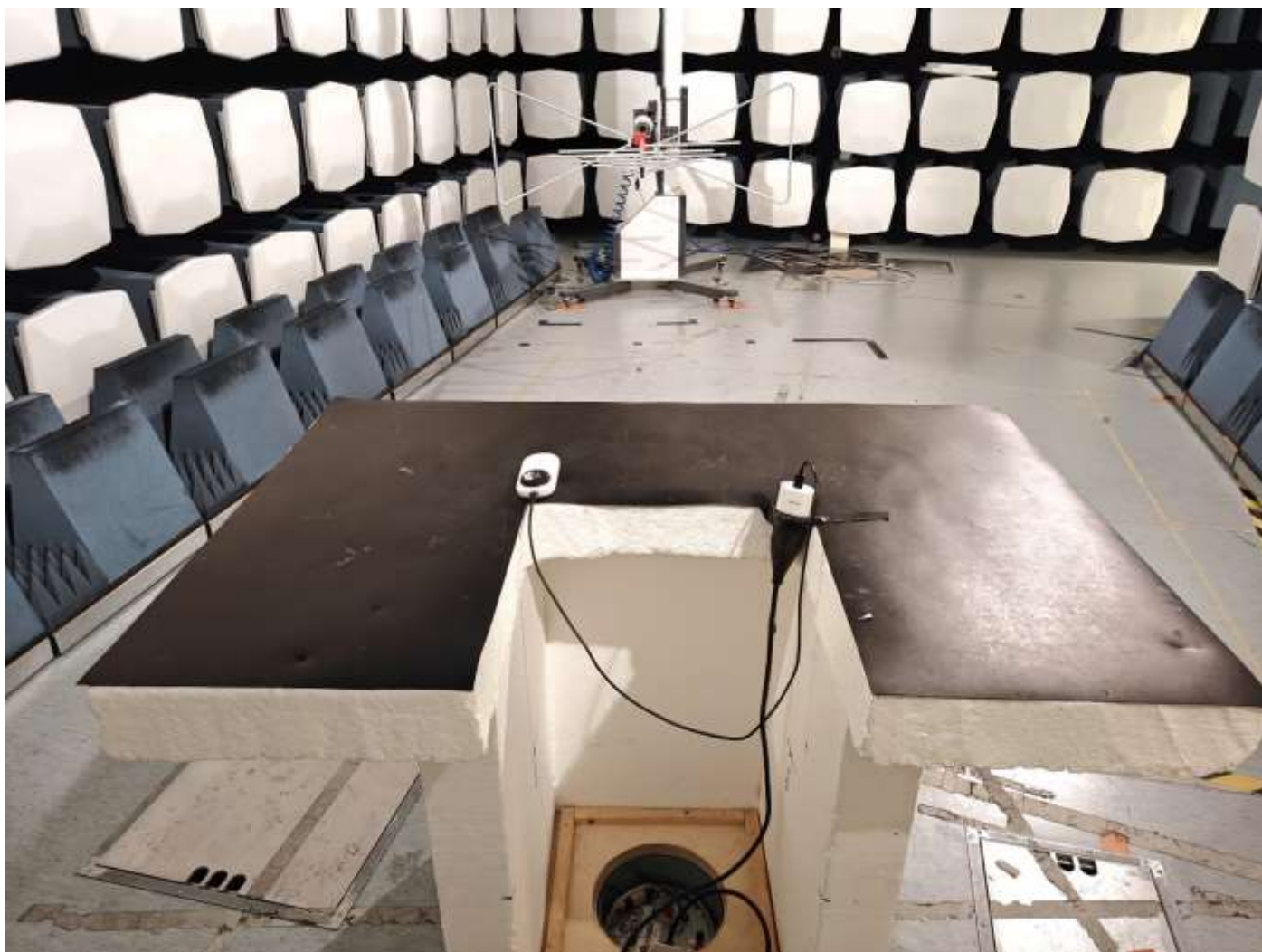
Picture 10 Radiated emission, view from EUT, 30 -1000 MHz
