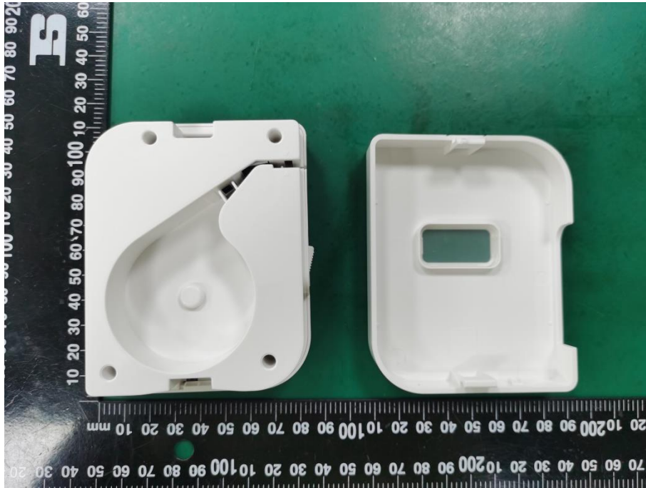
Internal Photo FCC ID: 2AWYK-HP1
