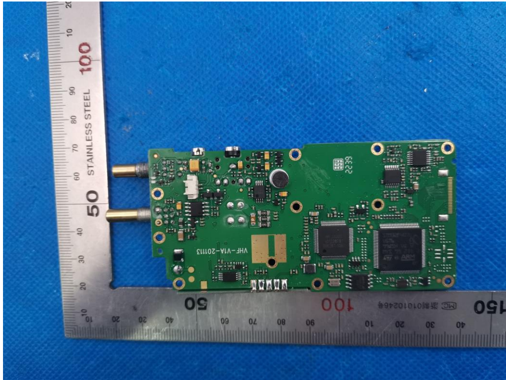
INTERNAL VIA OF EUT(FIGURE 3)
