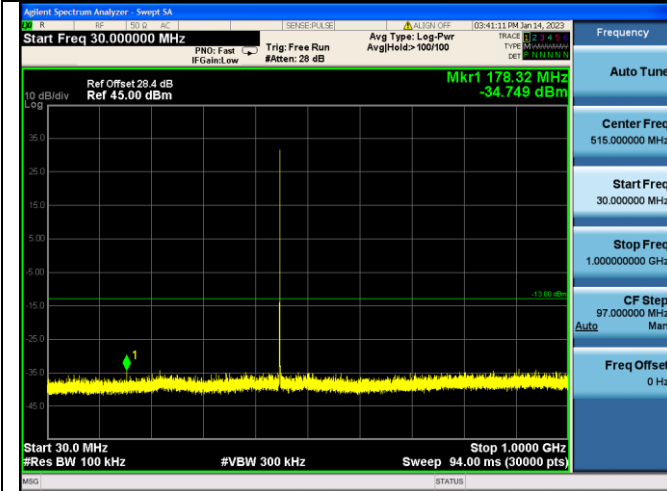
12.5kHz, FM modulation, Assigned Frequency:462.6500MHz, 2W
