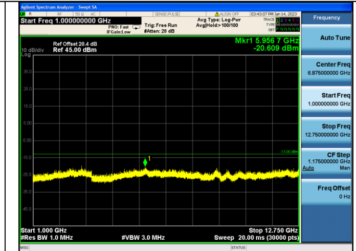
12.5kHz, FM modulation, Assigned Frequency:467.6500MHz, 2W
