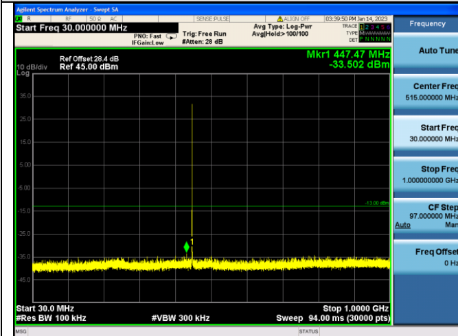
12.5kHz, FM modulation, Assigned Frequency:467.6500MHz, 2W
