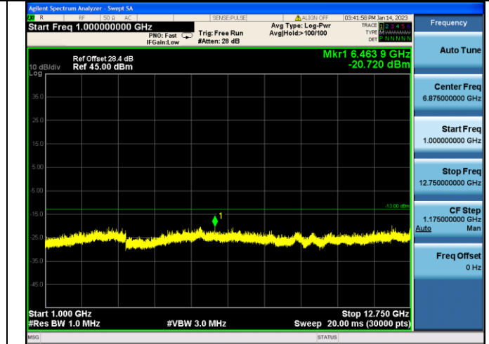
12.5kHz, FM modulation, Assigned Frequency:462.6500MHz, 2W
