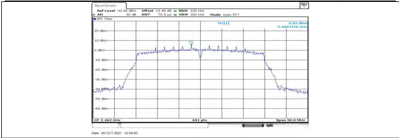
11N20MIMO Ant1_2462_0~Reference
