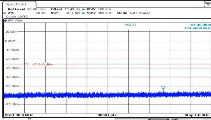
11G_Ant2_2412_0~Reference
