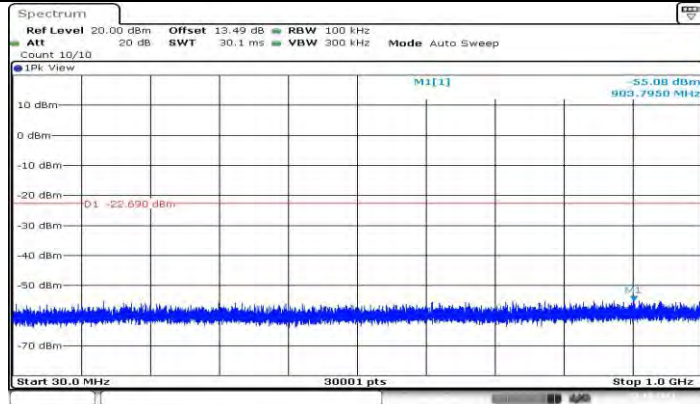
11B_Ant2_2412_0~Reference
