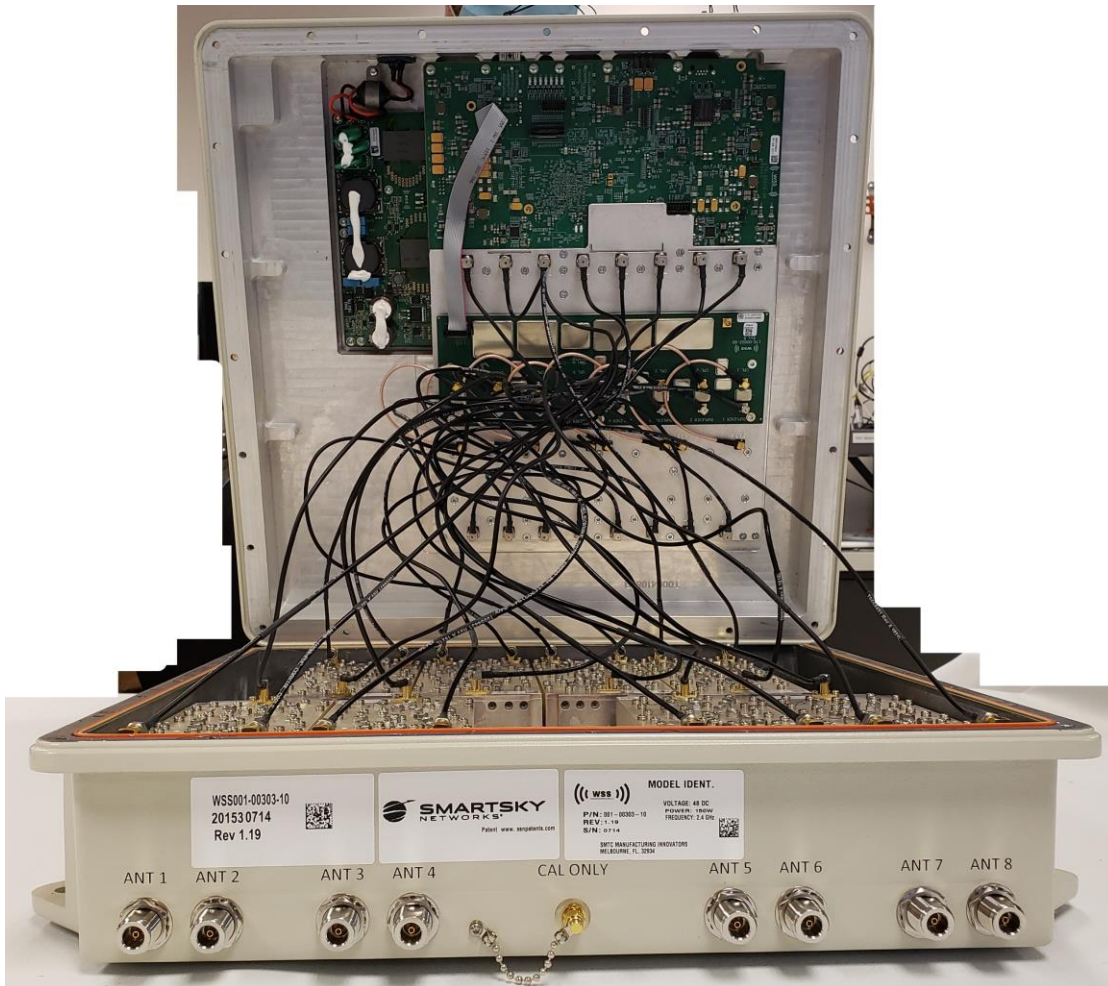
Figure 1 – RRH (fully installed)
