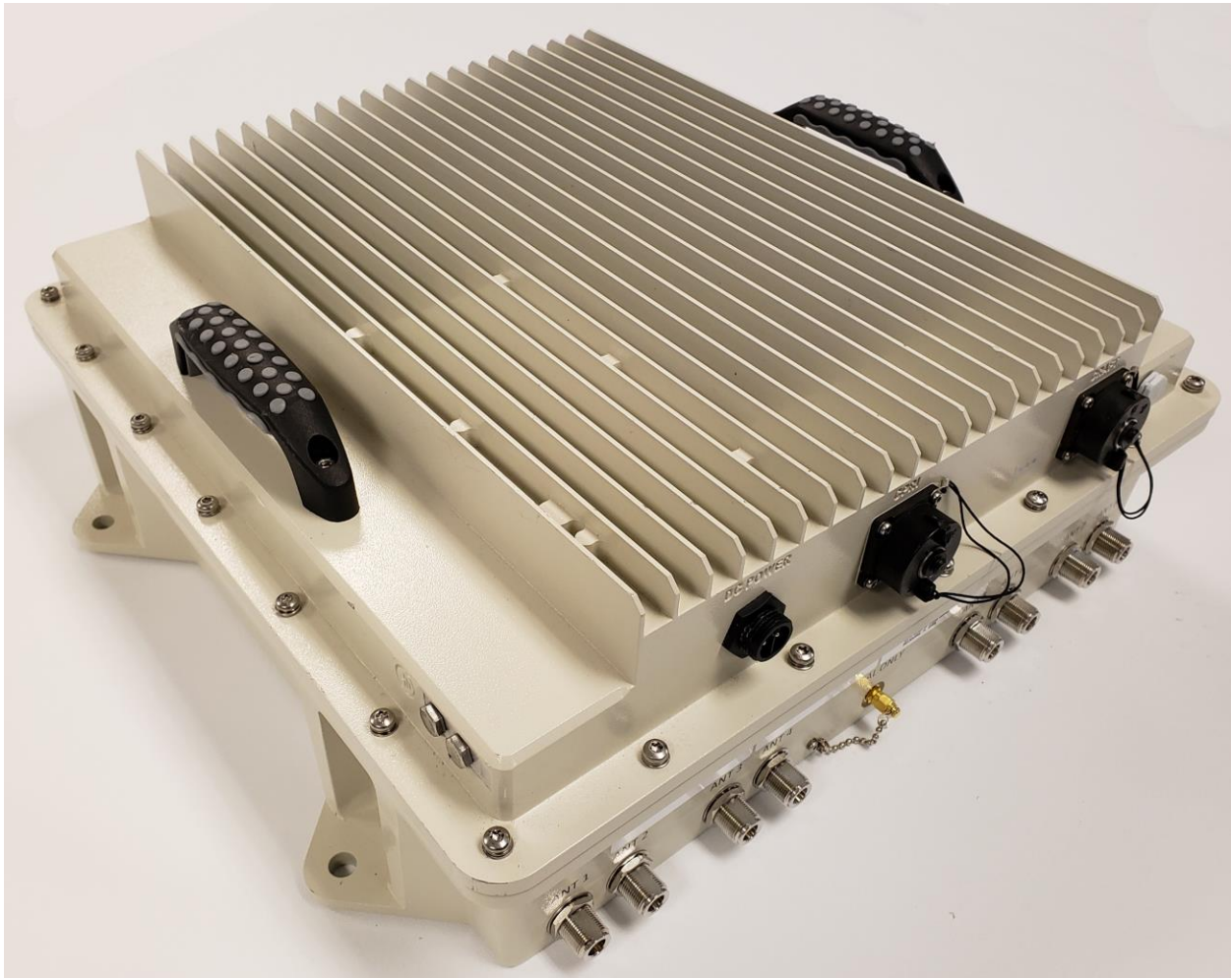
Figure 3 – RRH Top Left Side View
