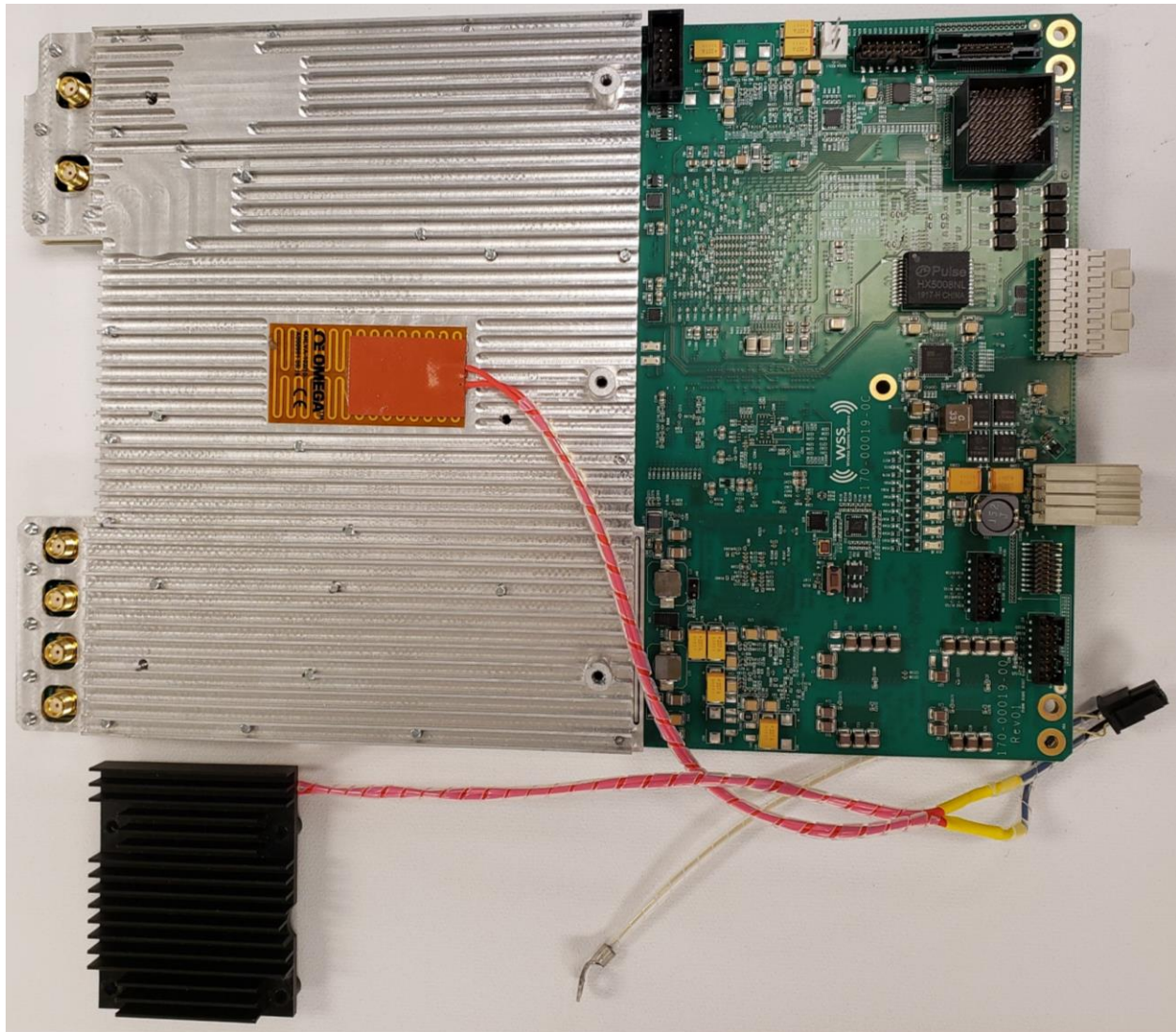
Figure 3 - ABR RF board (19 Board) Top view with shield and heaters
