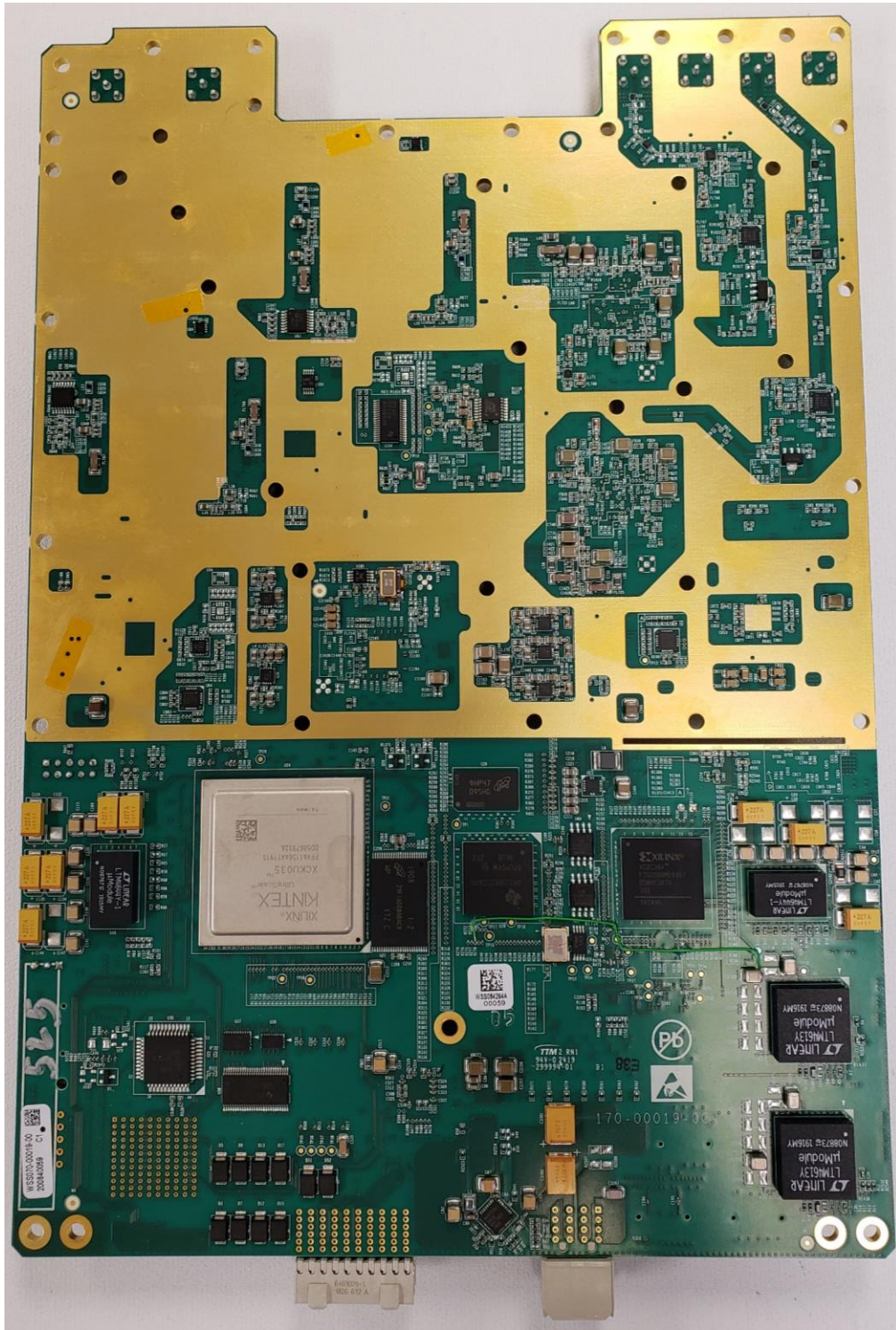
Figure 2 - ABR RF board (19 Board) Bottom view
