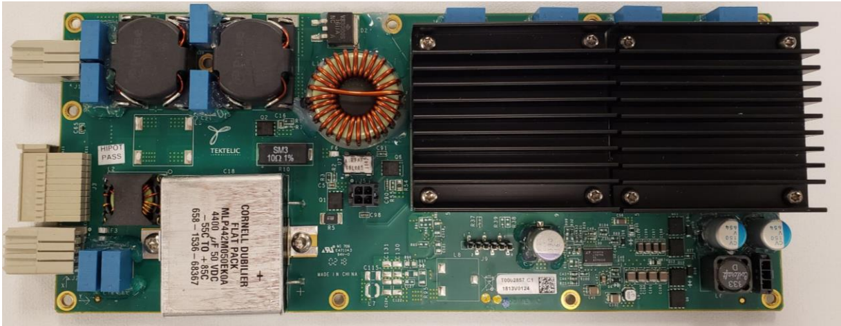
Figure 7 – Power Supply board Top view
