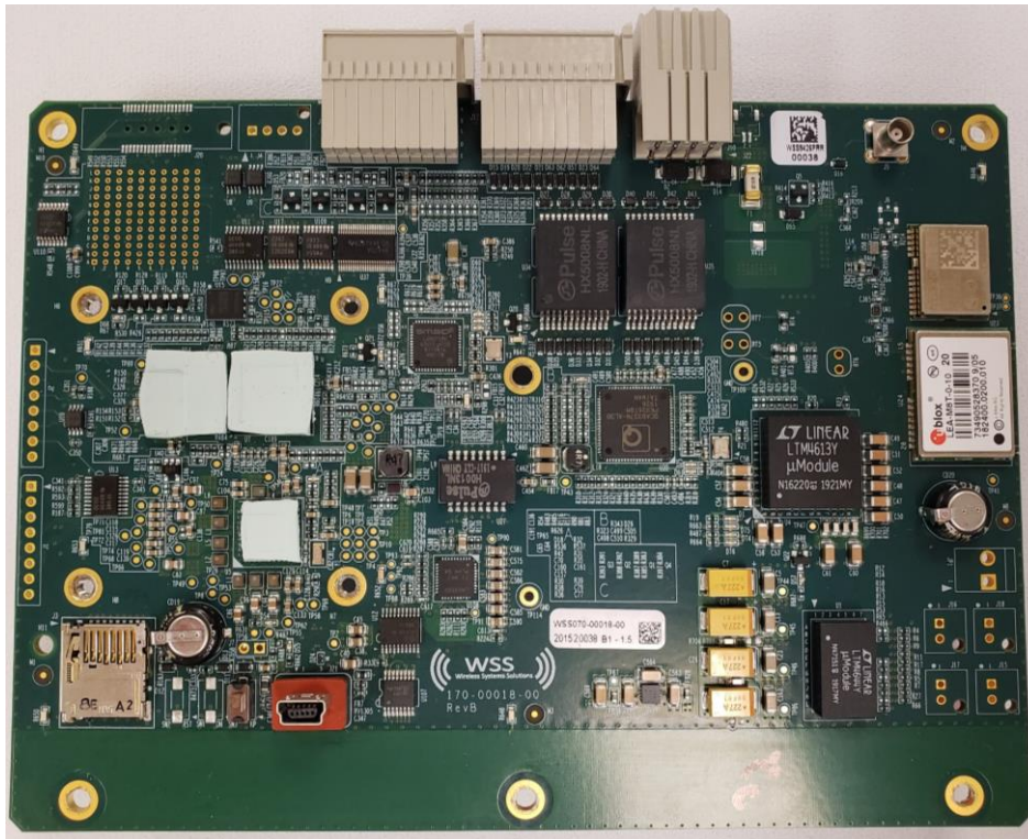
Figure 4 - ABR Digital board (18 Board) Top view
