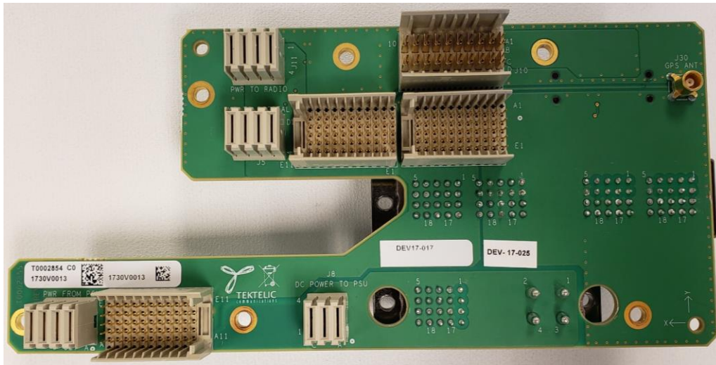
Figure 9 – Connector board Bottom view
