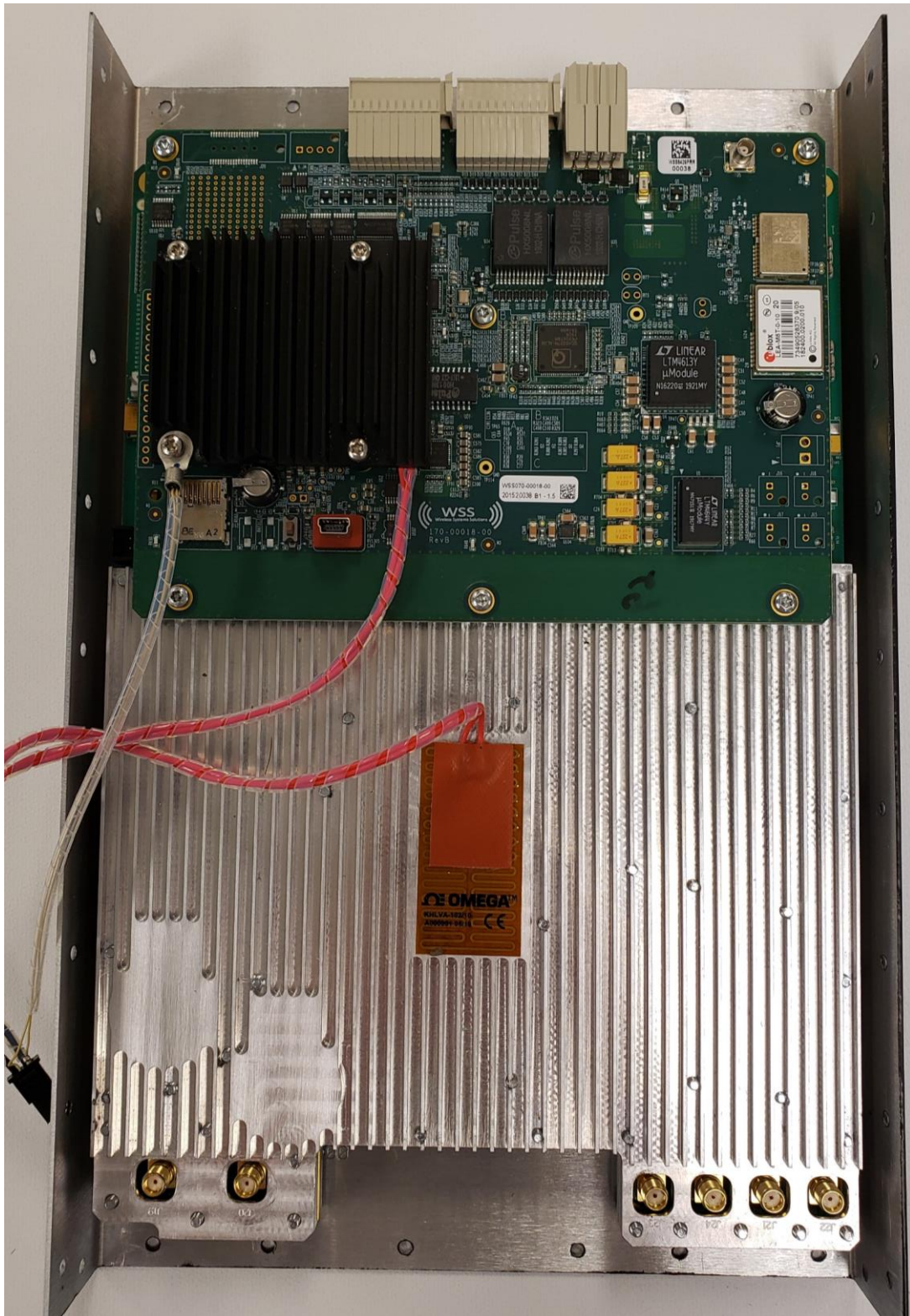
Figure 6 - ABR RF and Digital board (19 and 18 Board) + heaters
