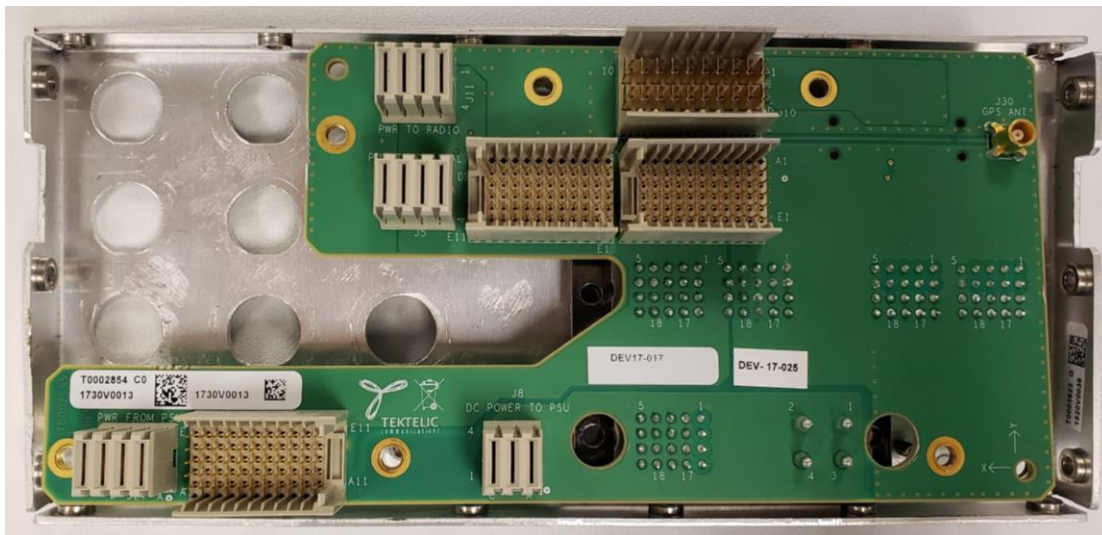
Figure 12 – Connector board in front-panel Top view
