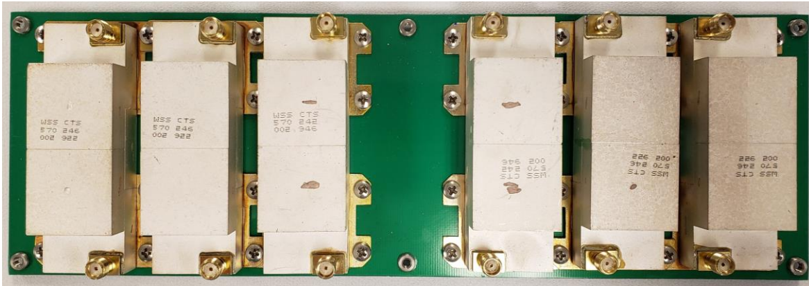
Figure 13 – Ceramic Filter board Top view
