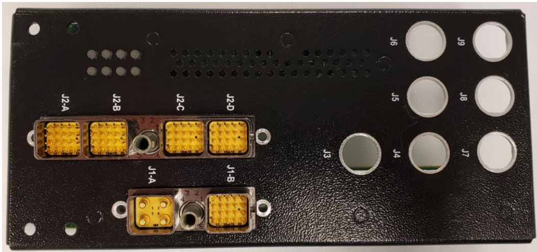
Figure 11 – Connector board in front-panel Top view
