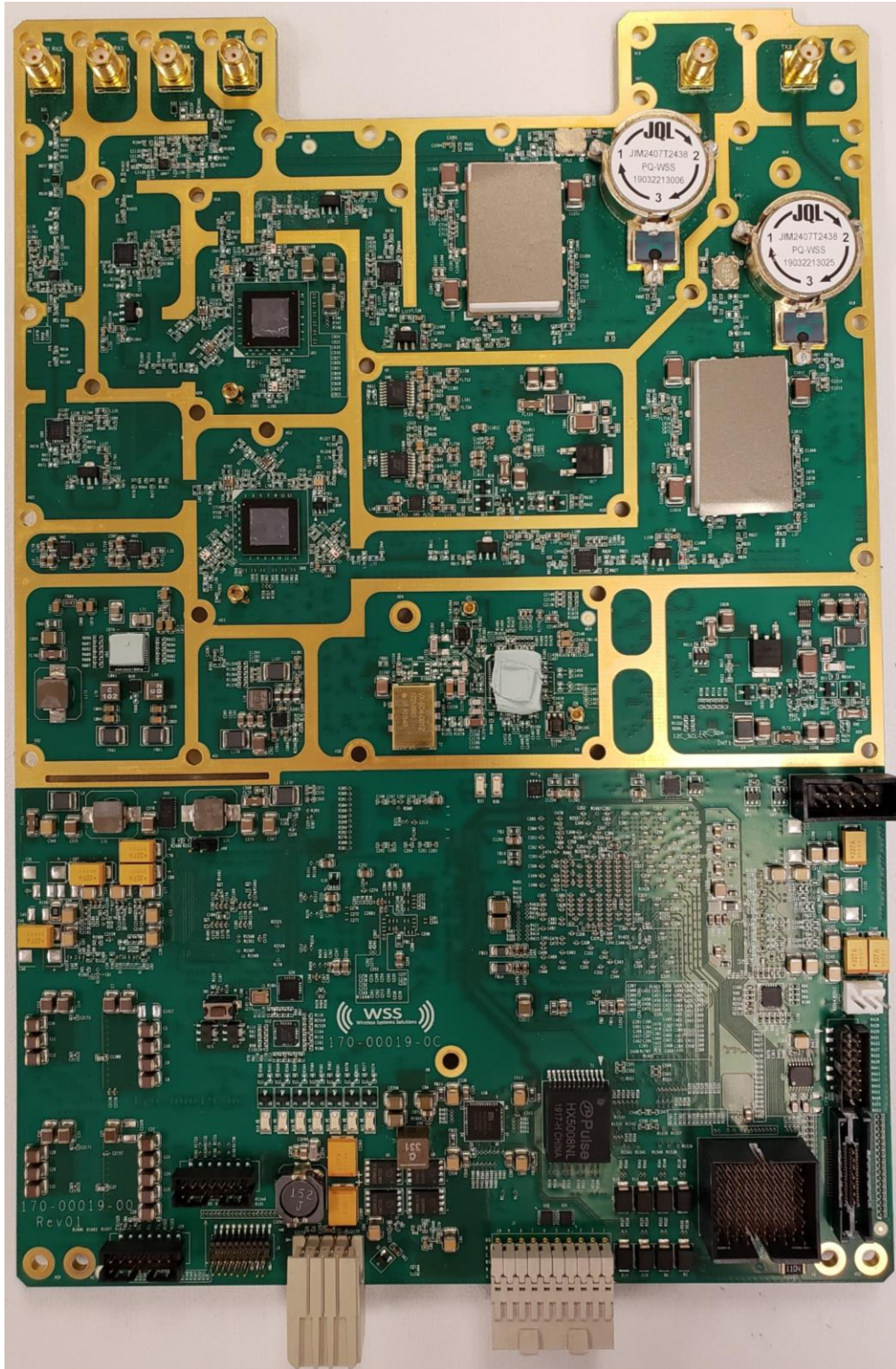
Figure 1 - ABR RF board (19 Board) Top view
