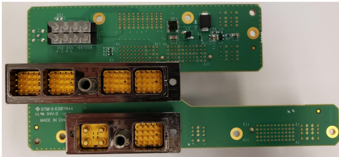
Figure 10 – Connector board Top view
