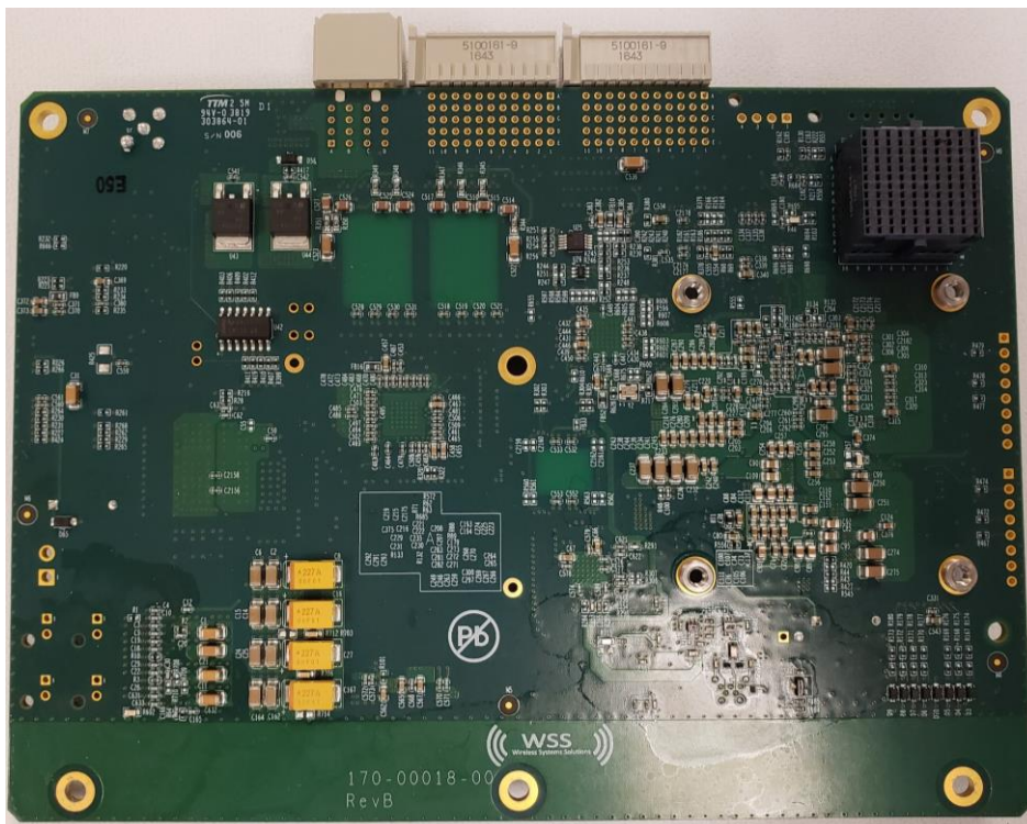
Figure 5 - ABR Digital board (18 Board) Bottom view
