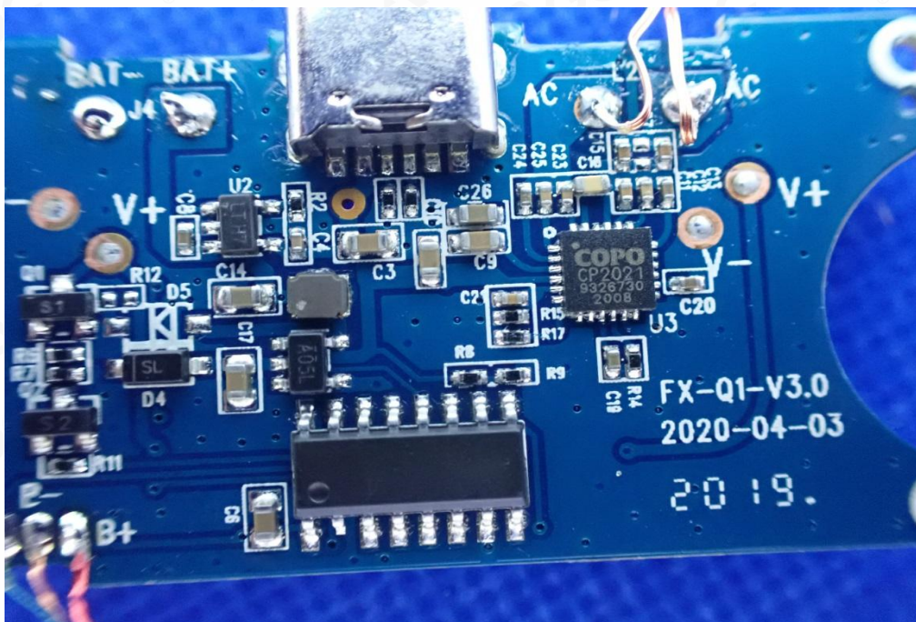
INTERNAL VIEW-6 OF Charging case
