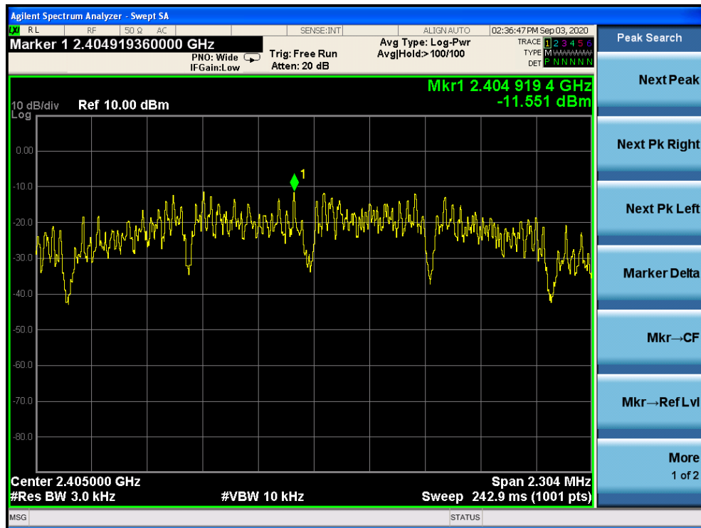
Power spectral density plot on 2405MHz 0.25Mbps
