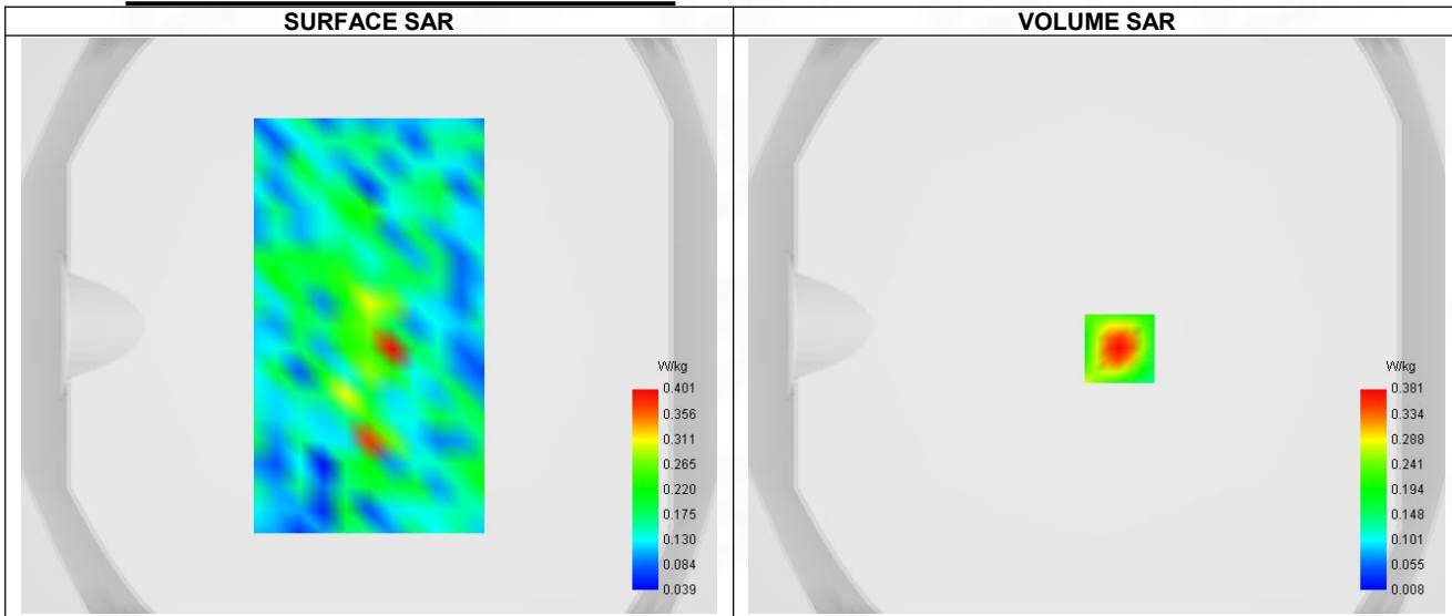
Maximum location: X=8.00, Y=-8.00 ; SAR Peak: 0.50 W/kg
