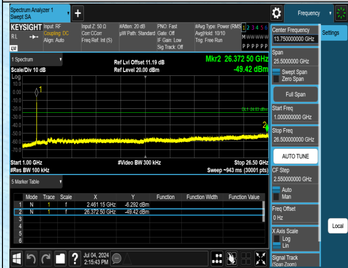
11N20SISO-Ant1-2462-1000~26500-PASS
