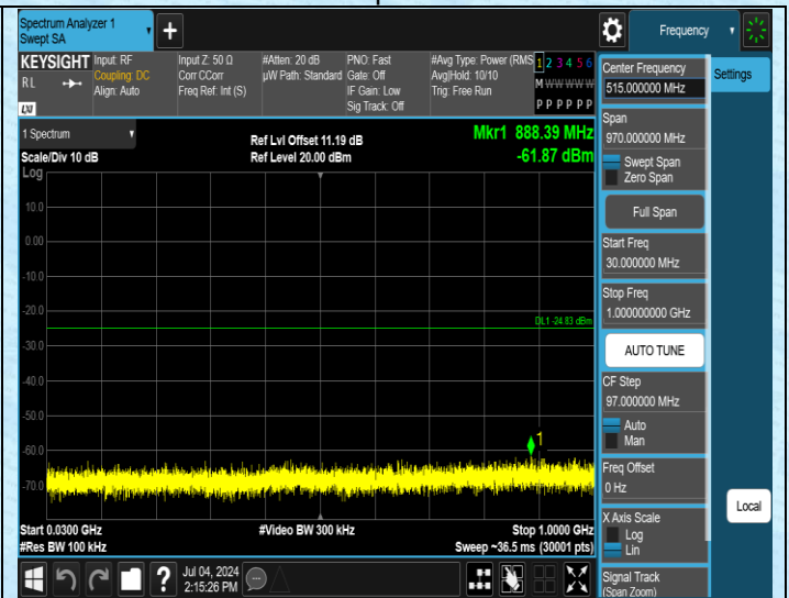
11N20SISO-Ant1-2462-30~1000-PASS
