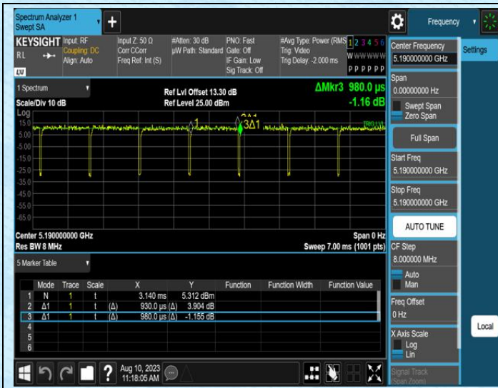
NTNV-11N40SISO-Ant1-5190
