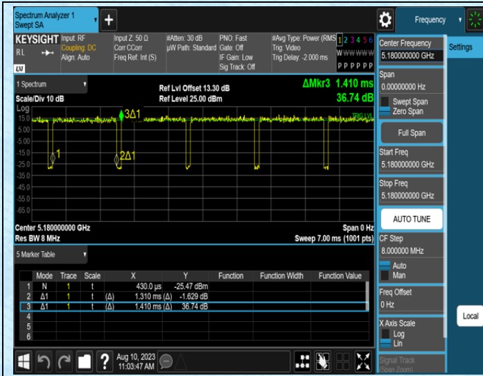
NTNV-11N20SISO-Ant1-5180
