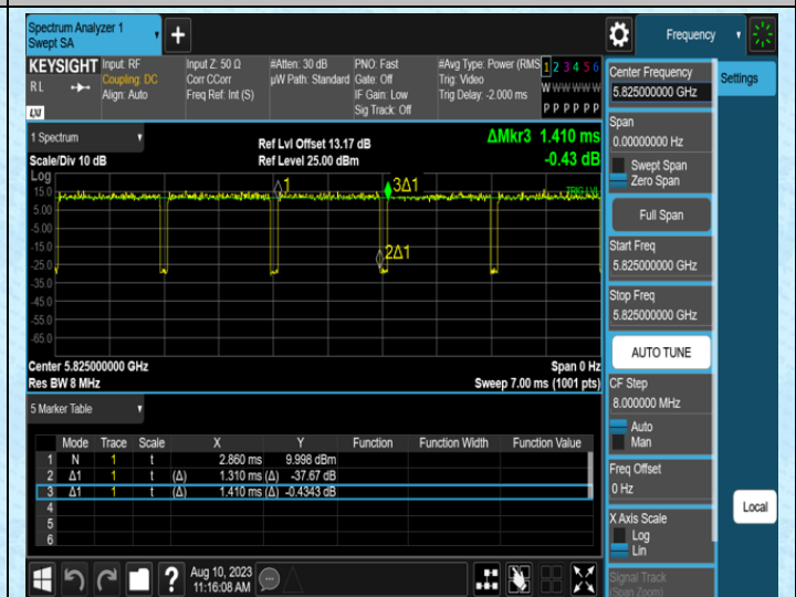
NTNV-11N20SISO-Ant1-5825
