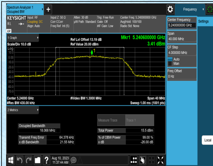
11AC20SISO-Ant1-5240
