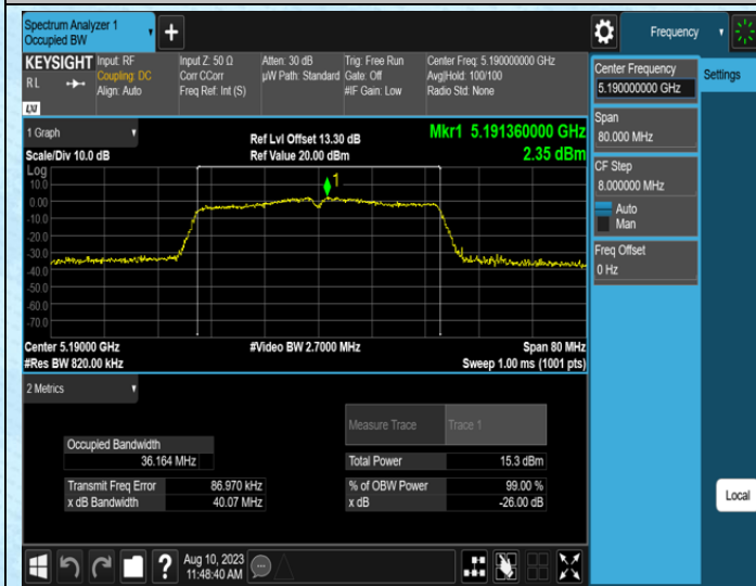
11AC40SISO-Ant1-5190
