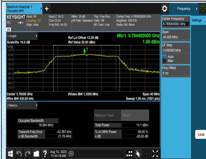
11AC20SISO-Ant1-5785
