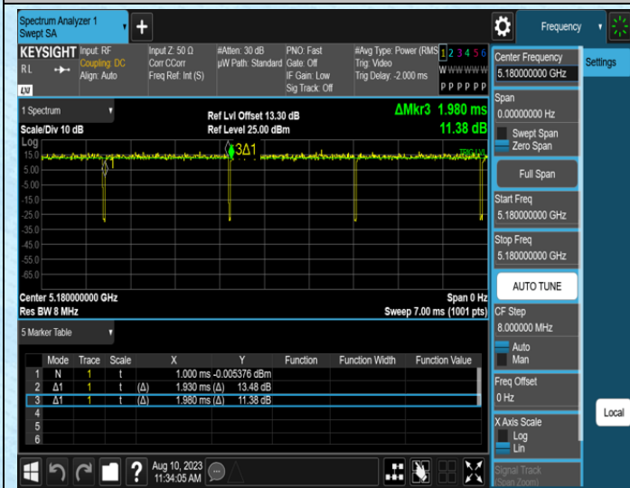
NTNV-11AC20SISO-Ant1-5180
