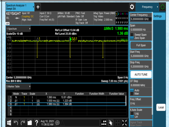
NTNV-11AC20SISO-Ant1-5200
