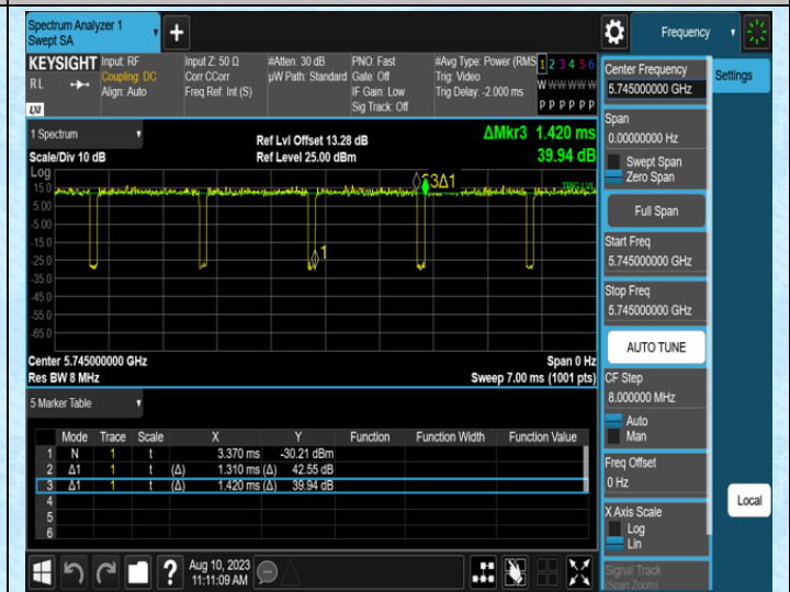
NTNV-11N20SISO-Ant1-5745
