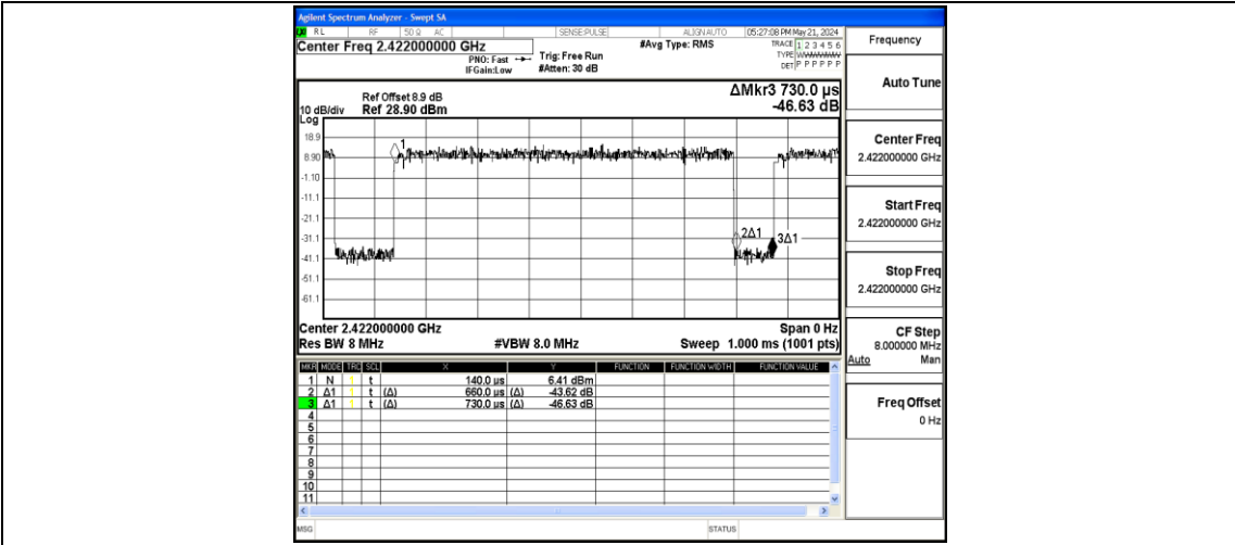
NTVN-11N40SISO-Ant1-2422
