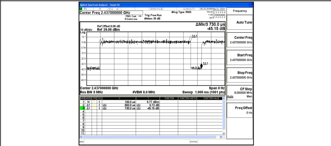
NTVN-11N40SISO-Ant1-2437
