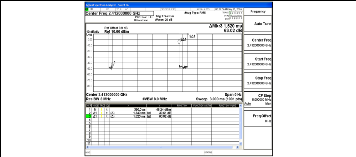
NTVN-11N20SISO-Ant1-2412
