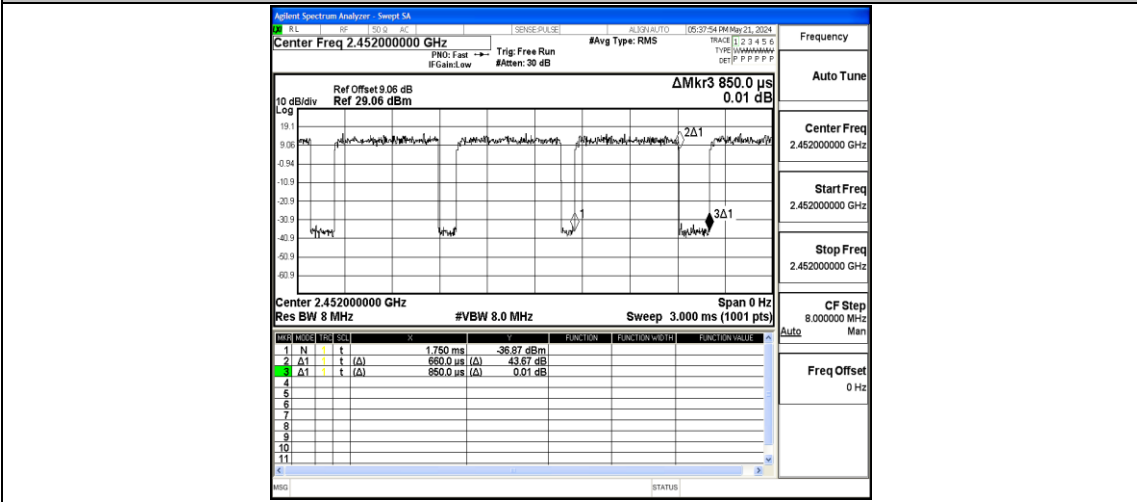
NTVN-11N40SISO-Ant1-2452
