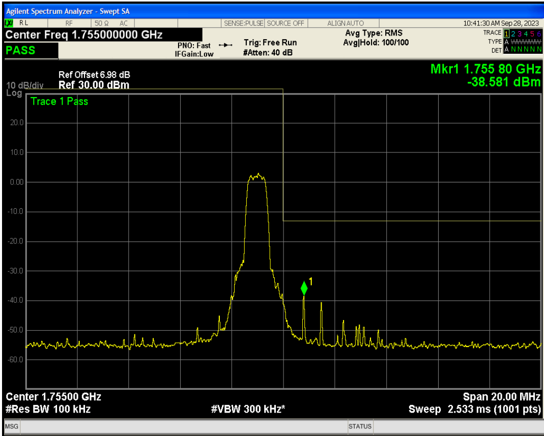
Band4 QAM16 BW=10MHz Channel=20350 RB Size=1 Position=#Max NB Index=7
