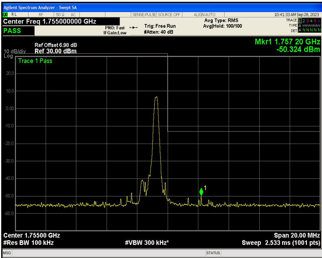
Band4 QAM16 BW=10MHz Channel=20350 RB Size=4 Position=#Max NB Index=7
