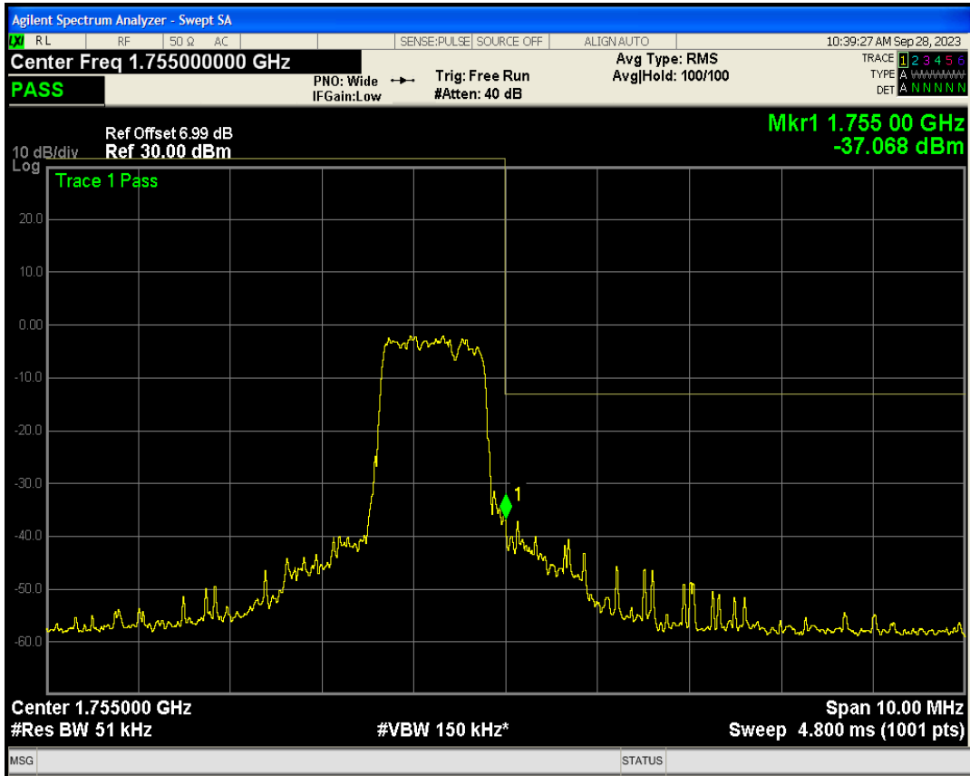
Band4 QAM16 BW=5MHz Channel=20375 RB Size=1 Position=#Max NB Index=3
