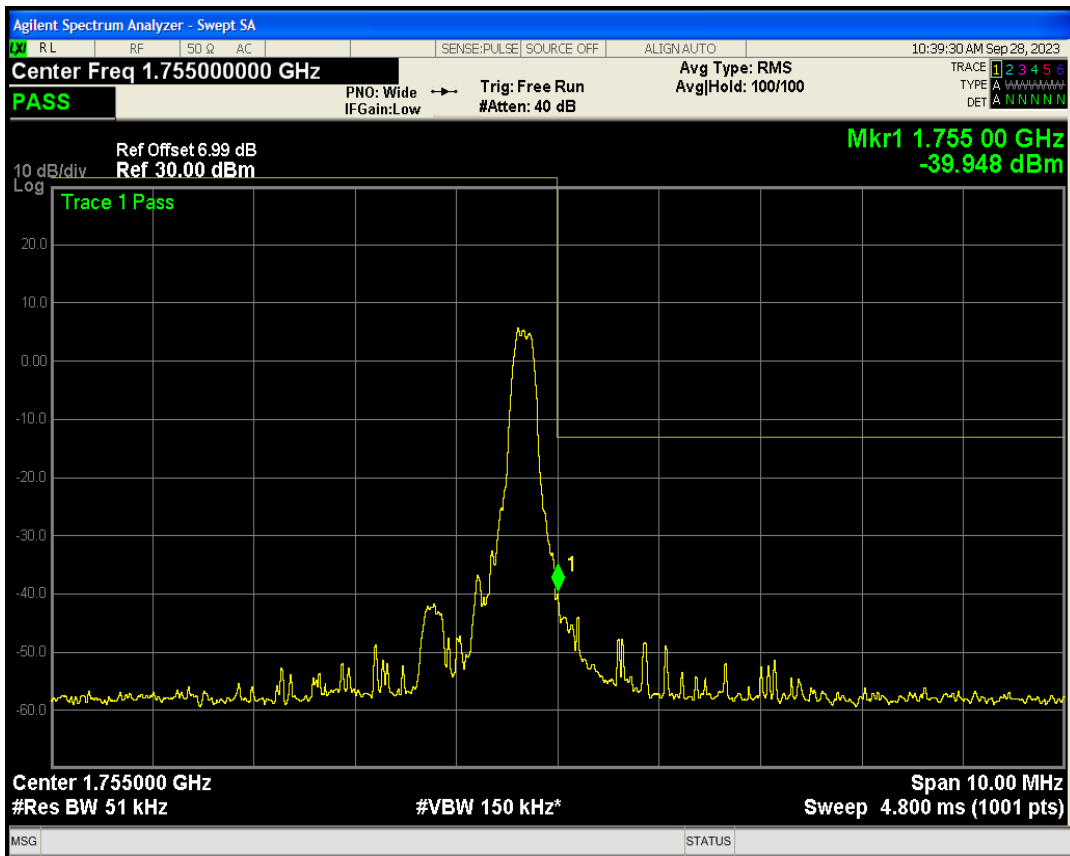
Band4 QAM16 BW=5MHz Channel=20375 RB Size=6 Position=#Max NB Index=3
