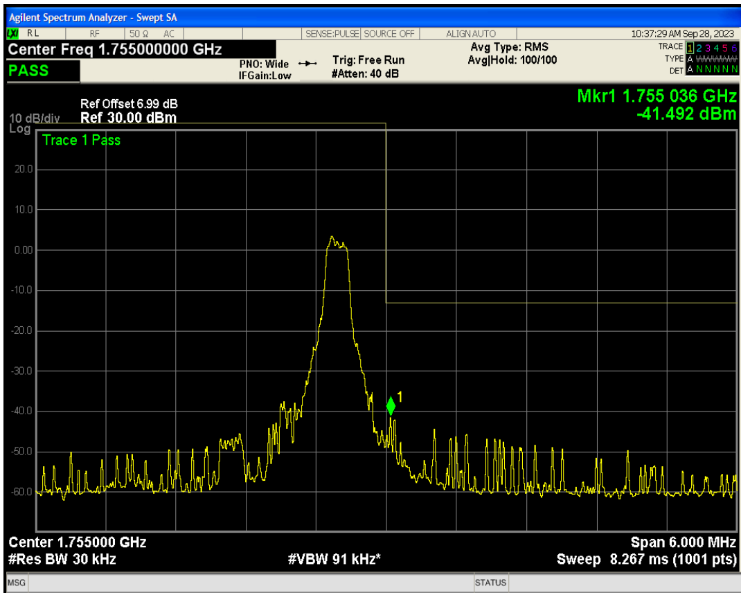
Band4 QPSK BW=3MHz Channel=20385 RB Size=6 Position=#Max NB Index=1
