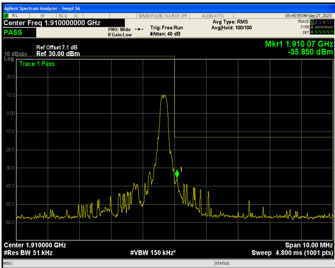
Band2 QPSK BW=5MHz Channel=19175 RB Size=6 Position=#Max NB Index=3
