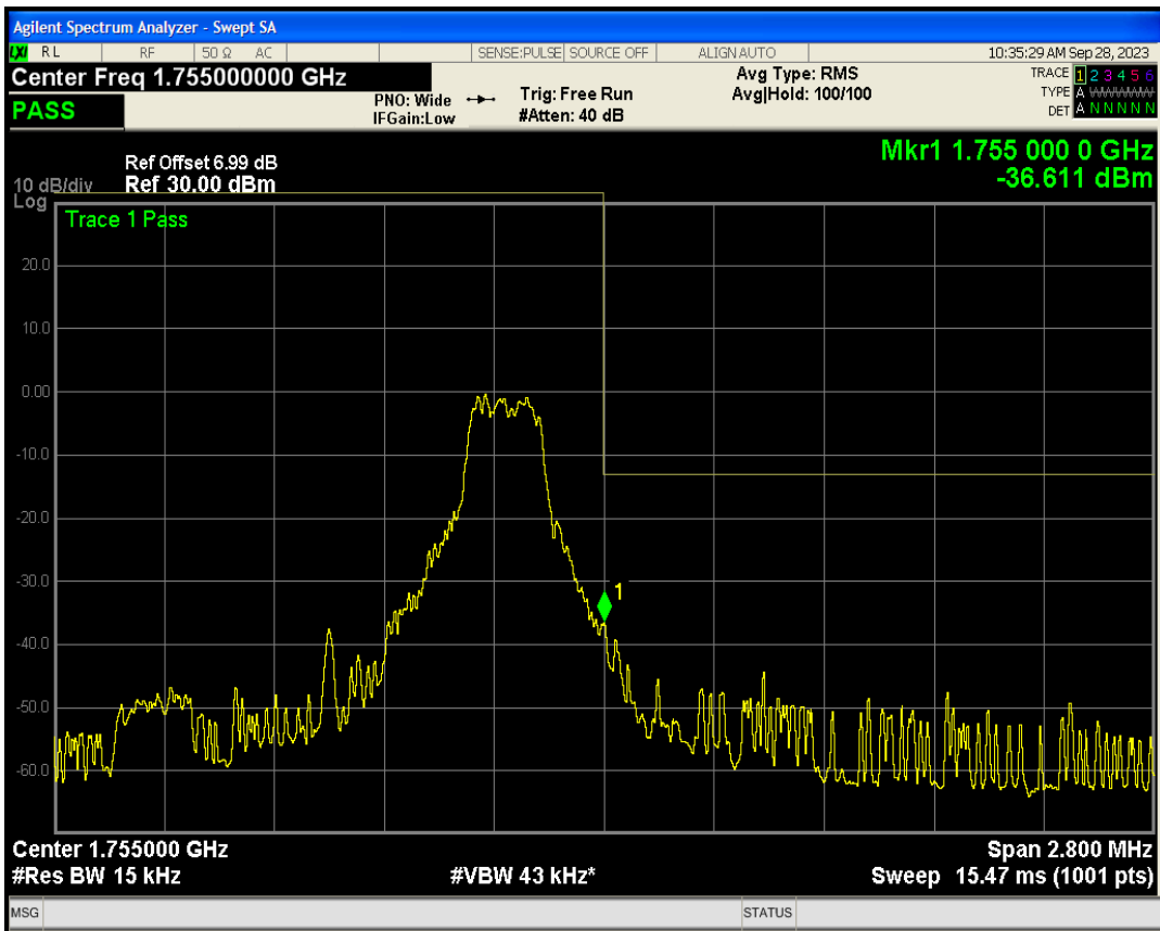
Band4 QAM16 BW=1.4MHz Channel=20393 RB Size=6 Position=#Max NB Index=0
