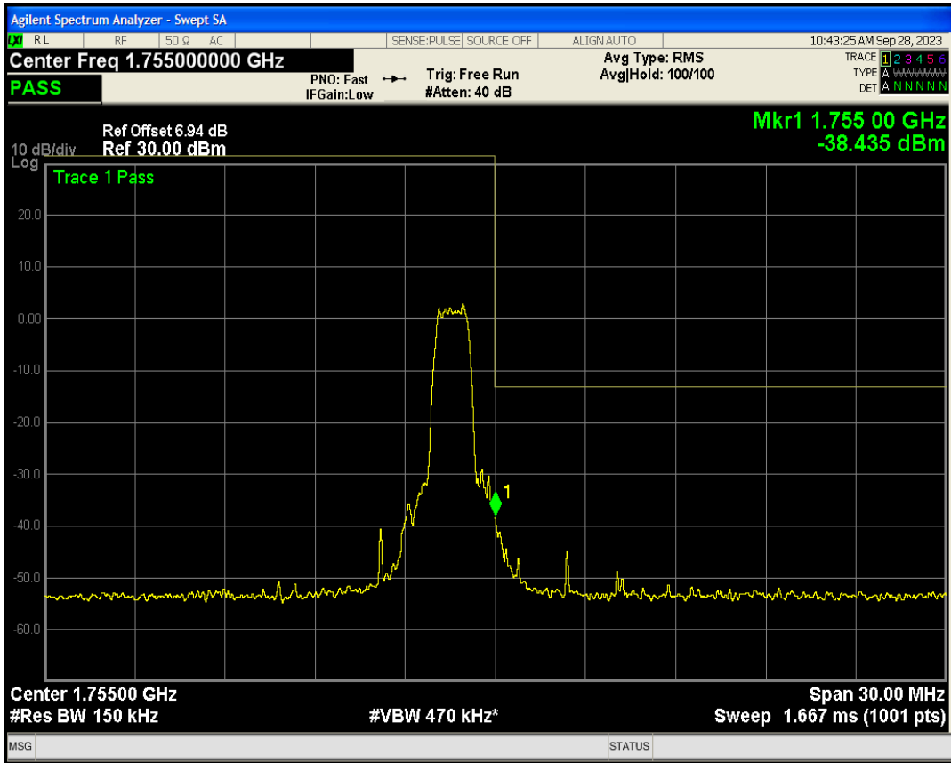
Band4 QAM16 BW=15MHz Channel=20325 RB Size=1 Position=#Max NB Index=11
