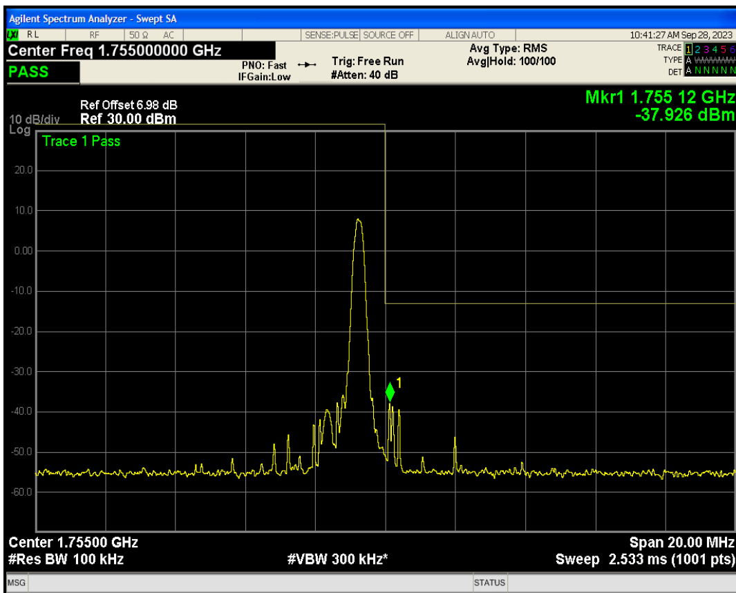
Band4 QPSK BW=10MHz Channel=20350 RB Size=4 Position=#Max NB Index=7
