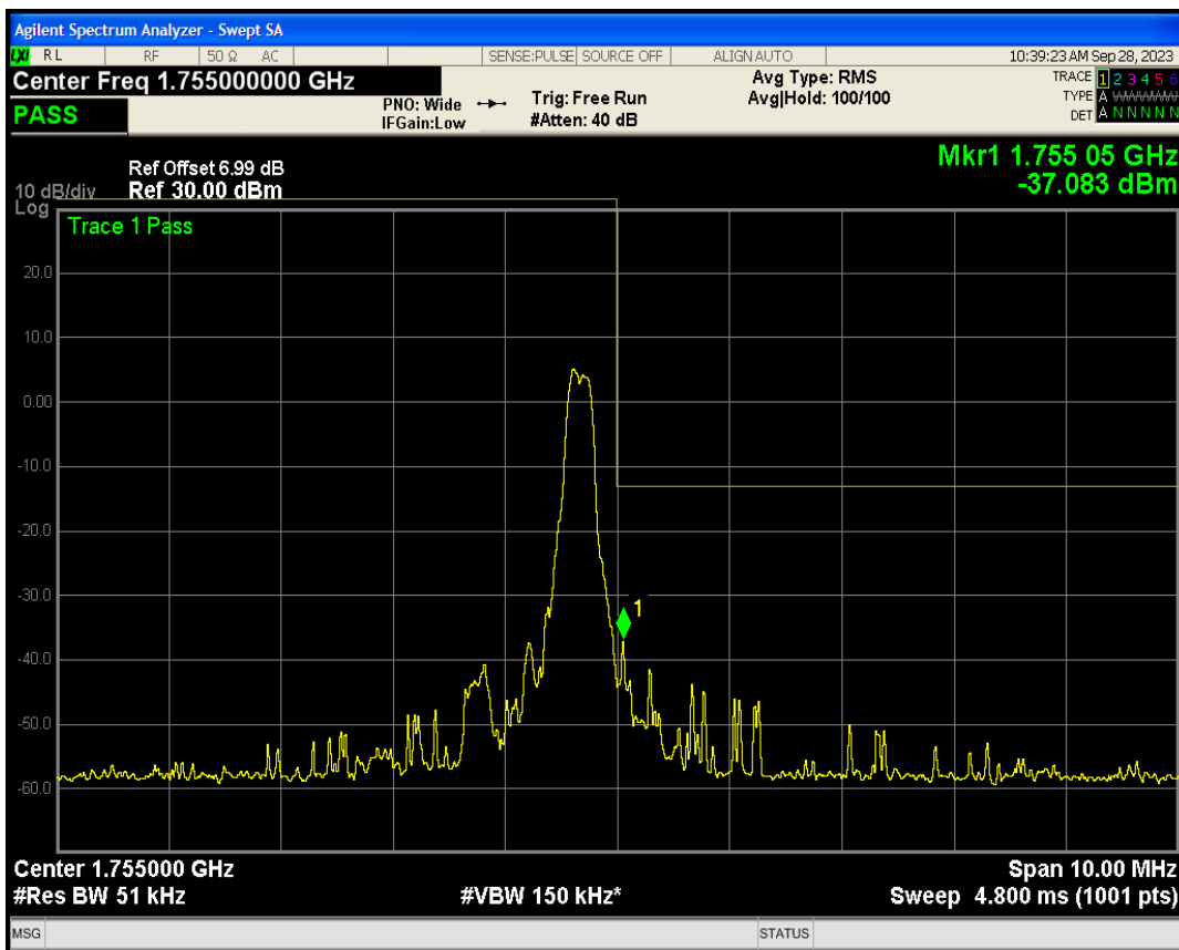
Band4 QPSK BW=5MHz Channel=20375 RB Size=6 Position=#Max NB Index=3
