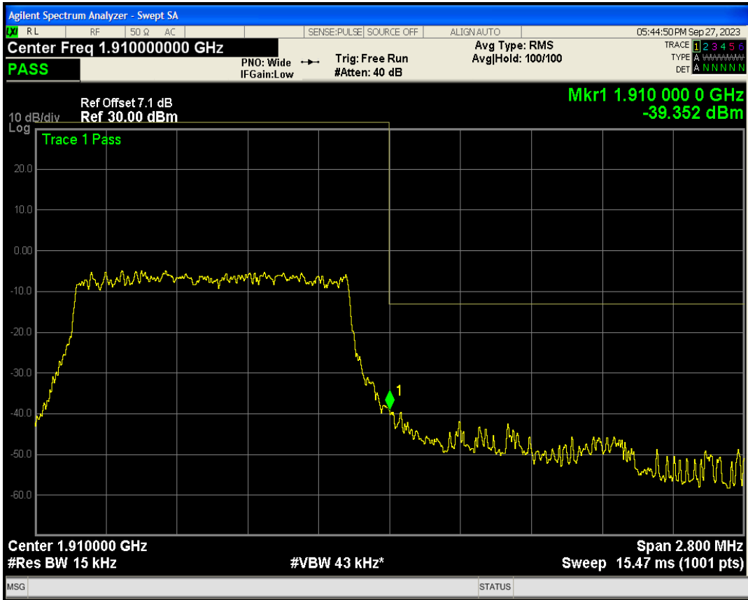
Band2 QAM16 BW=1.4MHz Channel=19193 RB Size=1 Position=#Max NB Index=0
