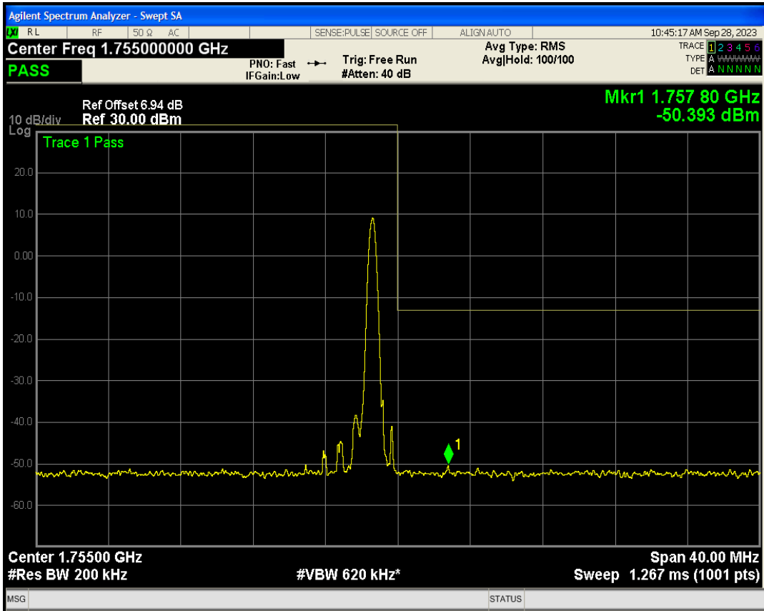
Band4 QAM16 BW=20MHz Channel=20300 RB Size=6 Position=#Max NB Index=15
