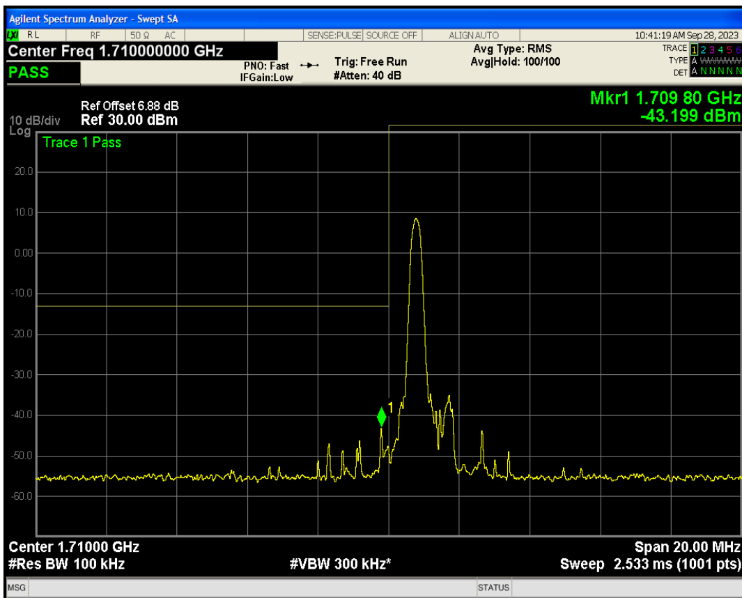
Band4 QAM16 BW=10MHz Channel=20000 RB Size=4 Position=#0 NB Index=0
