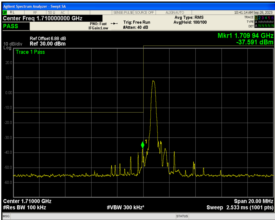
Band4 QPSK BW=10MHz Channel=20000 RB Size=4 Position=#0 NB Index=0
