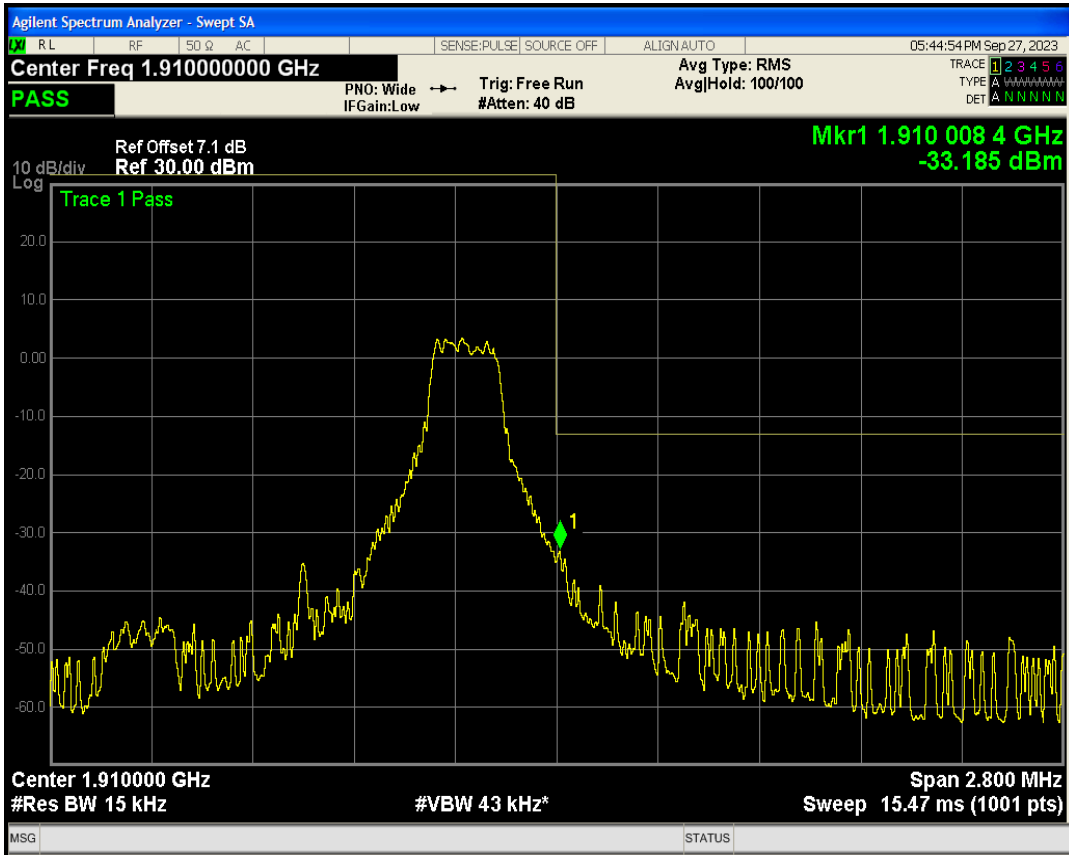
Band2 QAM16 BW=1.4MHz Channel=19193 RB Size=6 Position=#Max NB Index=0
