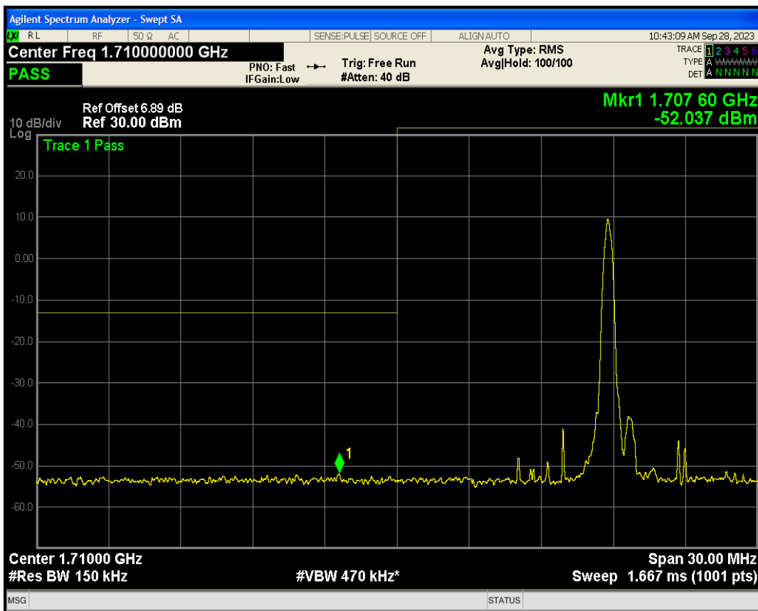
Band4 QPSK BW=15MHz Channel=20025 RB Size=6 Position=#0 NB Index=7
