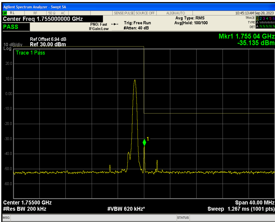
Band4 QPSK BW=20MHz Channel=20300 RB Size=6 Position=#Max NB Index=15
