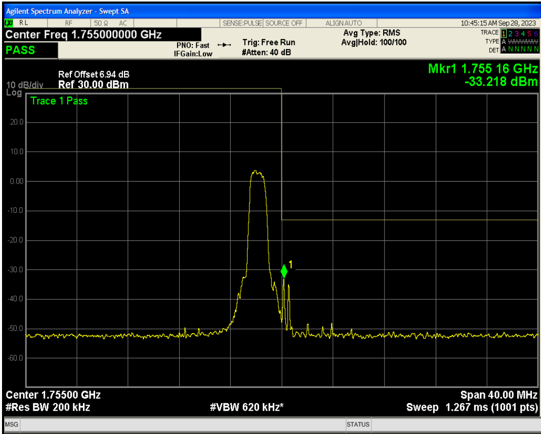
Band4 QAM16 BW=20MHz Channel=20300 RB Size=1 Position=#Max NB Index=15
