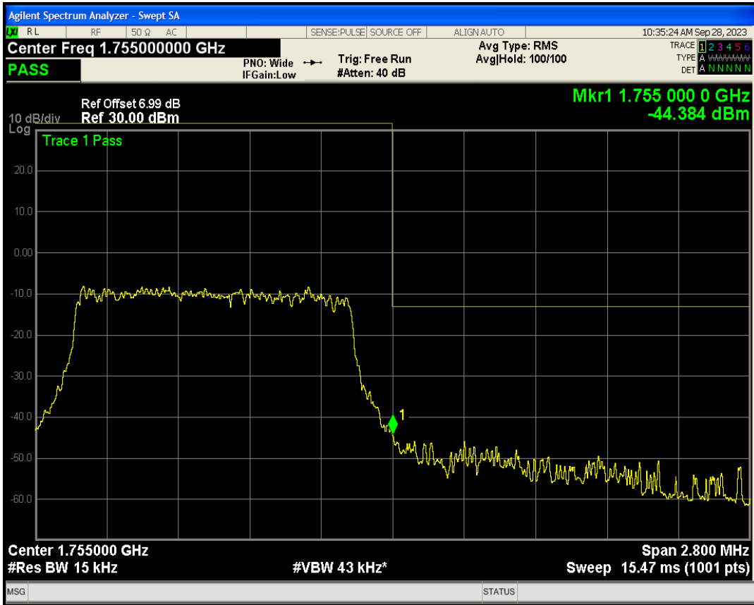
Band4 QAM16 BW=1.4MHz Channel=20393 RB Size=1 Position=#Max NB Index=0
