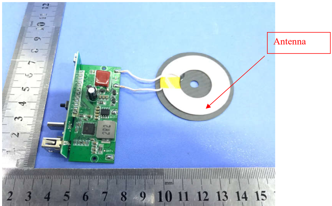
Photo 7 Appearance of PCB
