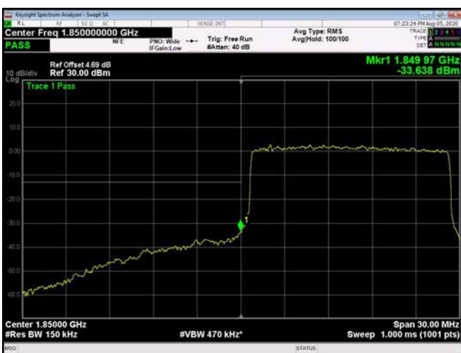
15MHz / 64QAM / Low Channel / Full RB
