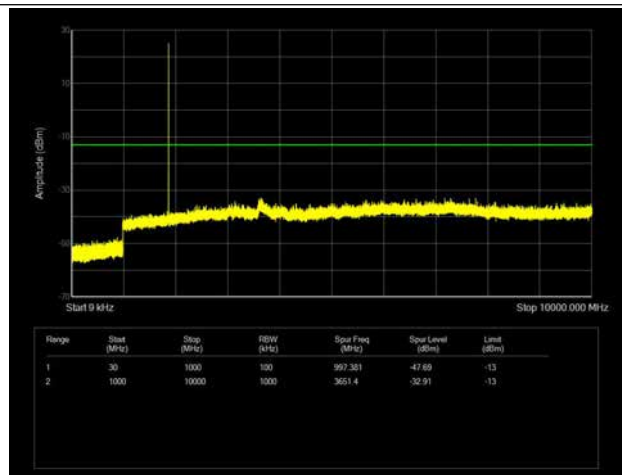
LTE Band 2 _ 1.4MHz BW _ Middle Channel
