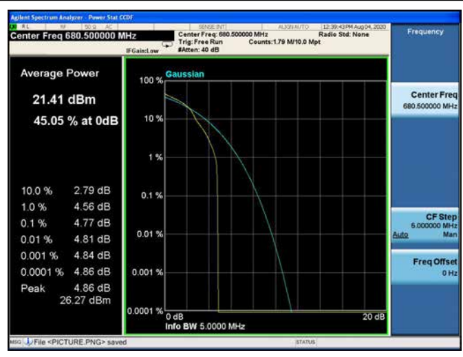
5MHz / 64QAM / Middle Channel
