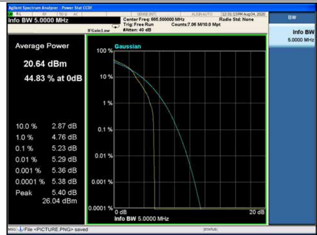
5MHz / QPSK / Middle Channel
