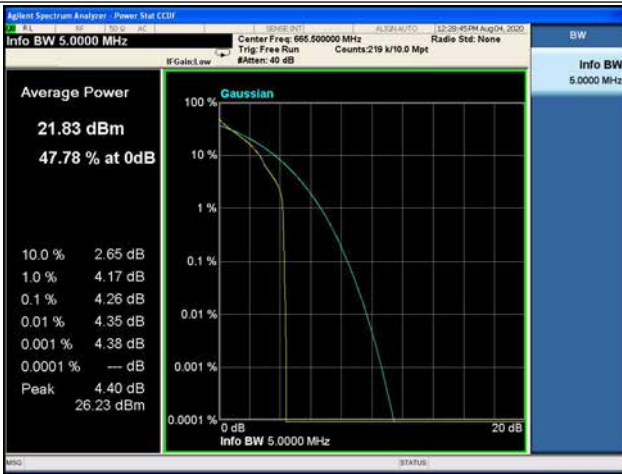
5MHz / 64QAM / Low Channel
