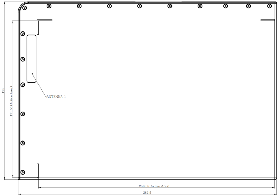
Figure E-1 Antenna Location (Rear Side View)
