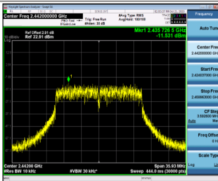
11N20SISO_Ant1_2442
