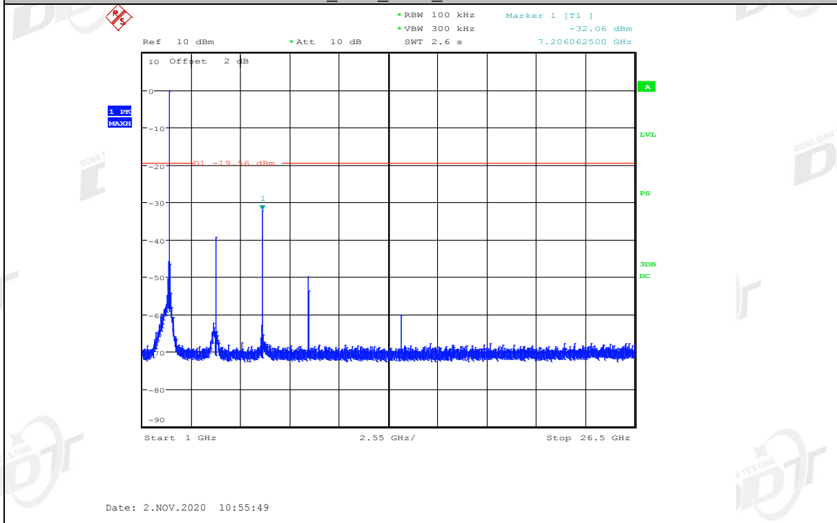
BLE_Ant1_2440_0~Reference
