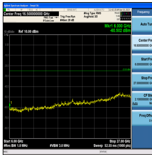
Band7-15MHz-QPSK-21100-75RB#0-Range3:6000~27000MHz
