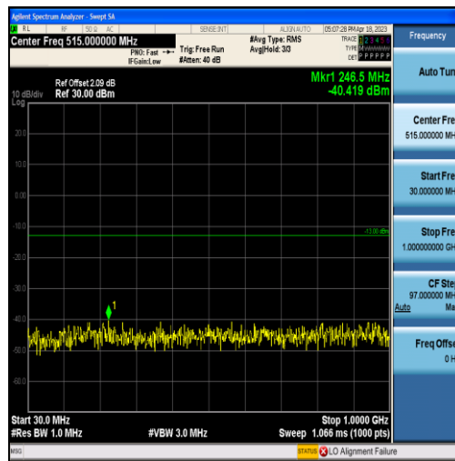
Band4-5MHz-16QAM-19975-25RB#0-Range1:30~1000MHz
