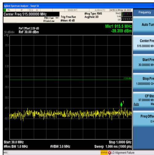
Band4-3MHz-QPSK-20175-15RB#0-Range1:30~1000MHz
