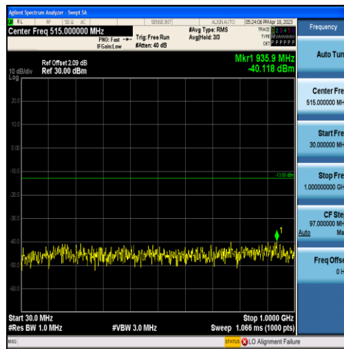
Band4-10MHz-16QAM-20000-50RB#0-Range1:30~1000MHz
