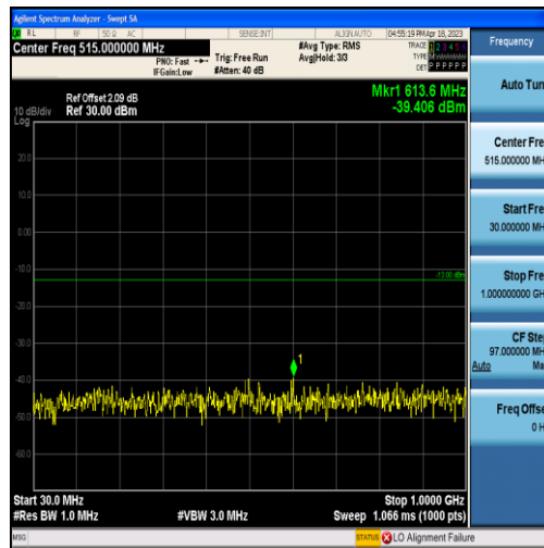
Band4-3MHz-16QAM-20175-15RB#0-Range1:30~1000MHz
