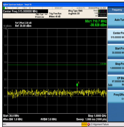
Band4-5MHz-QPSK-20375-25RB#0-Range1:30~1000MHz
