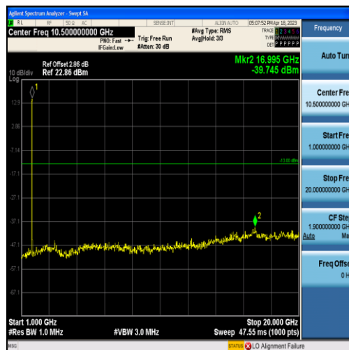
Band4-5MHz-16QAM-20175-25RB#0-Range2:1000~20000MHz
