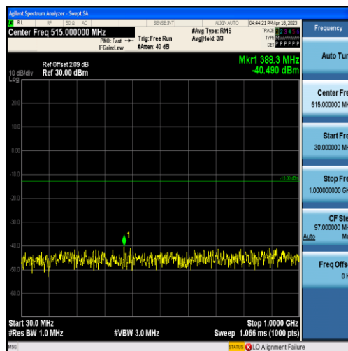
Band4-1.4MHz-16QAM-20393-6RB#0-Range1:30~1000MHz
