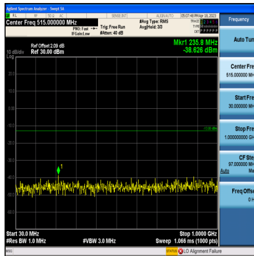
Band4-5MHz-16QAM-20175-25RB#0-Range1:30~1000MHz
