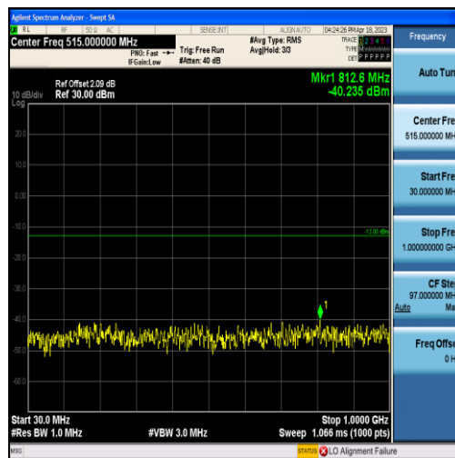
Band2-15MHz-QPSK-18900-75RB#0-Range1:30~1000MHz
