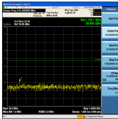
Band4-3MHz-QPSK-20385-15RB#0-Range1:30~1000MHz
