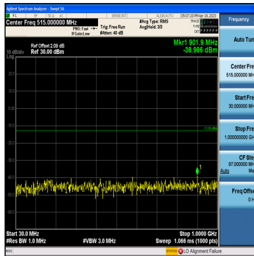
Band4-5MHz-QPSK-19975-25RB#0-Range1:30~1000MHz
