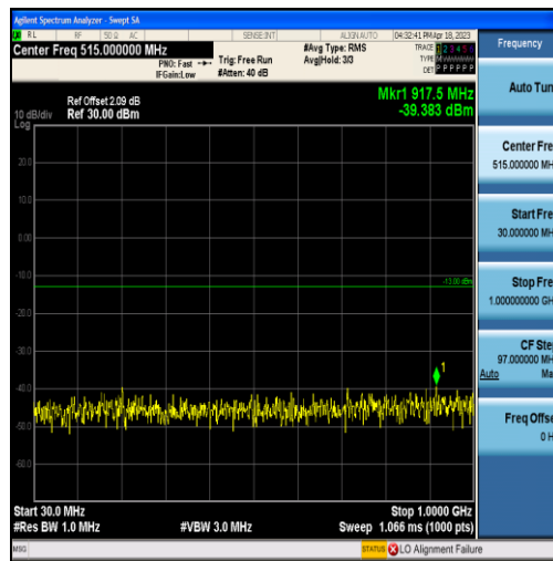
Band2-20MHz-16QAM-18700-100RB#0-Range1:30~1000MHz
