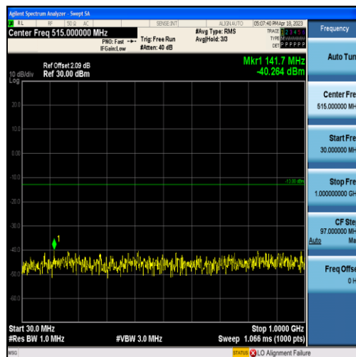
Band4-5MHz-QPSK-20175-25RB#0-Range1:30~1000MHz
