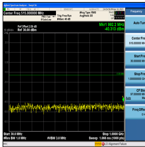
Band4-3MHz-16QAM-19965-15RB#0-Range1:30~1000MHz
