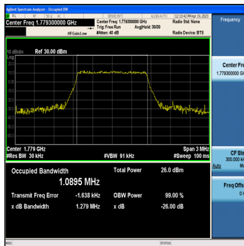
Band66-1.4MHz-16QAM-132665-6RB#0-1.0895
