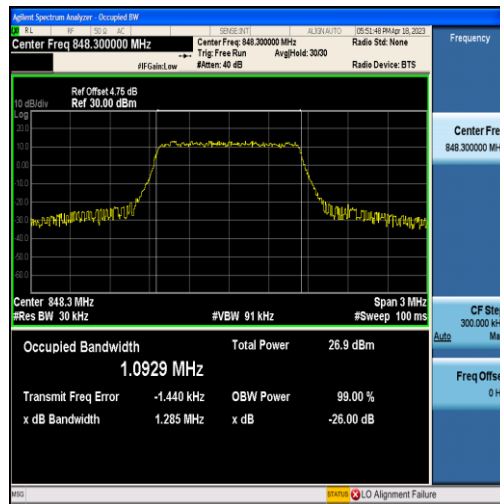
Band5-1.4MHz-QPSK-20643-6RB#0-1.0929
