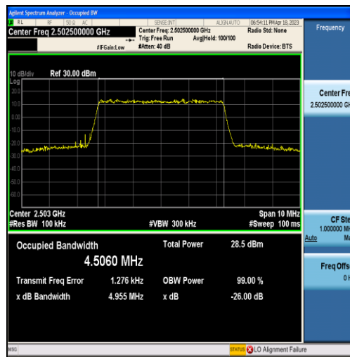
Band7-5MHz-QPSK-20775-25RB#0-4.5060
