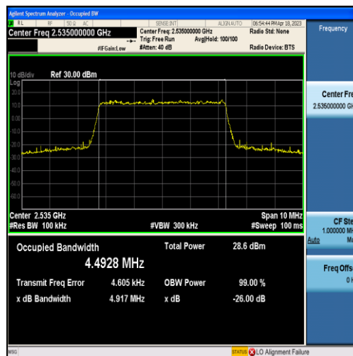
Band7-5MHz-QPSK-21100-25RB#0-4.4928
