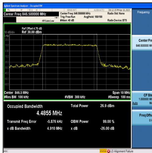
Band5-5MHz-16QAM-20625-25RB#0-4.4855
