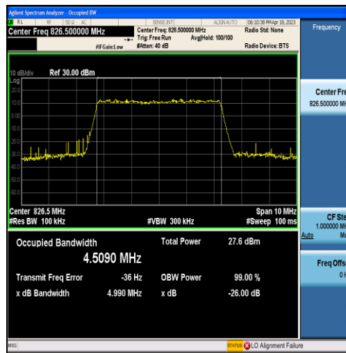
Band5-5MHz-QPSK-20425-25RB#0-4.5090
