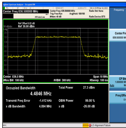
Band5-5MHz-16QAM-20525-25RB#0-4.4846
