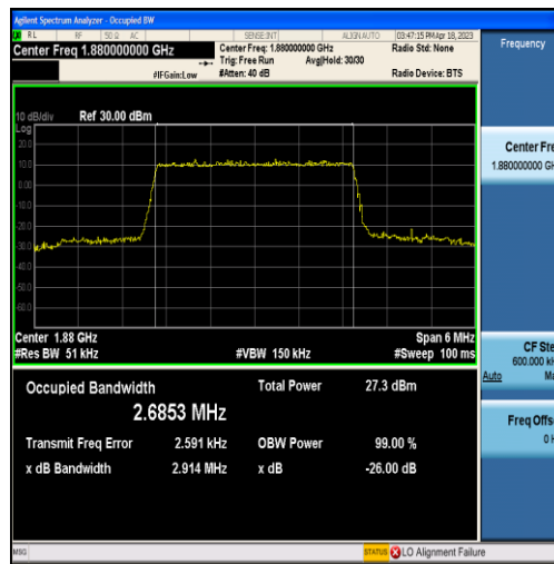
Band2-3MHz-16QAM-18900-15RB#0-2.6853
