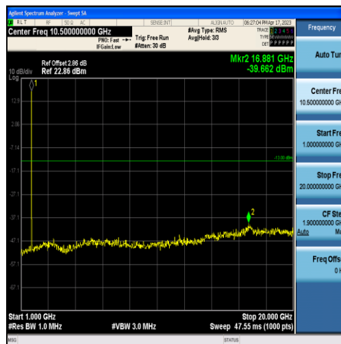
Band66-3MHz-QPSK-132322-15RB#0-Range2:1000~20000MHz
