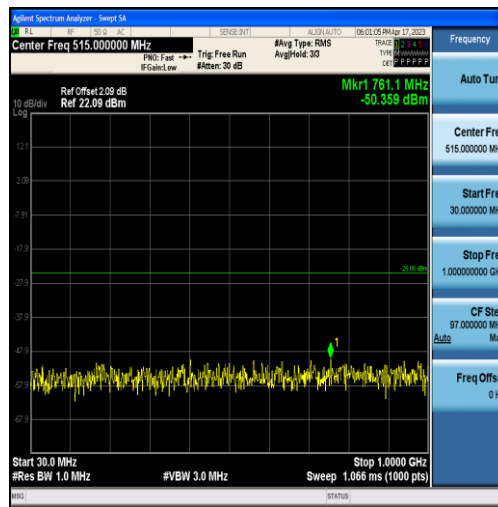
Band7-20MHz-16QAM-21100-60RB#0-Range1:30~1000MHz
