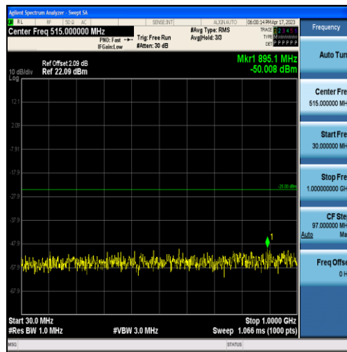
Band7-20MHz-16QAM-20850-60RB#0-Range1:30~1000MHz
