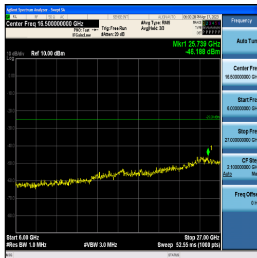
Band7-20MHz-16QAM-20850-60RB#0-Range3:6000~27000MHz
