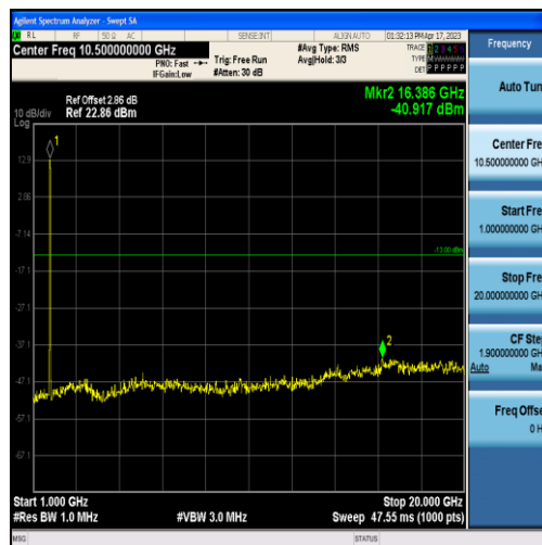
Band4-10MHz-16QAM-20350-50RB#0-Range2:1000~20000MHz
