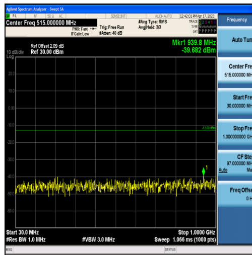
Band2-15MHz-16QAM-18900-75RB#0-Range1:30~1000MHz
