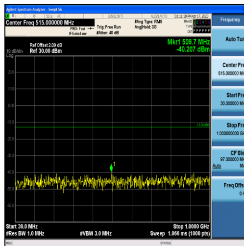
Band4-3MHz-QPSK-20385-15RB#0-Range1:30~1000MHz
