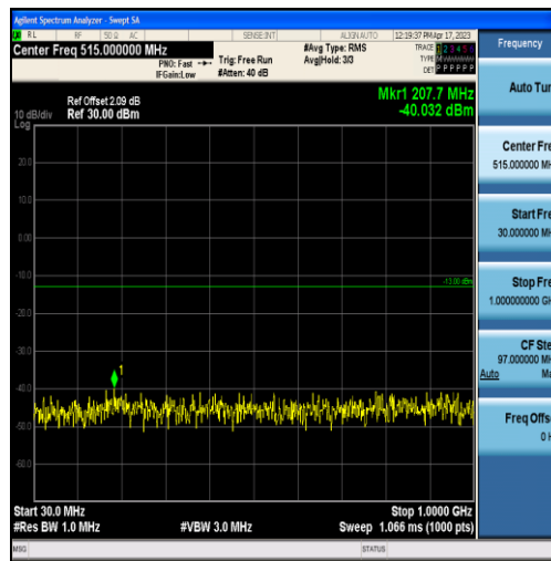
Band2-5MHz-16QAM-18900-25RB#0-Range1:30~1000MHz
