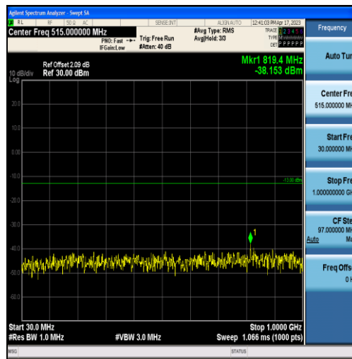
Band2-15MHz-QPSK-18675-75RB#0-Range1:30~1000MHz
