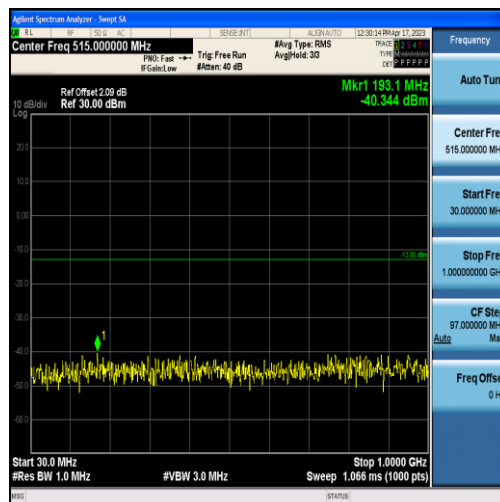
Band2-10MHz-QPSK-19150-50RB#0-Range1:30~1000MHz
