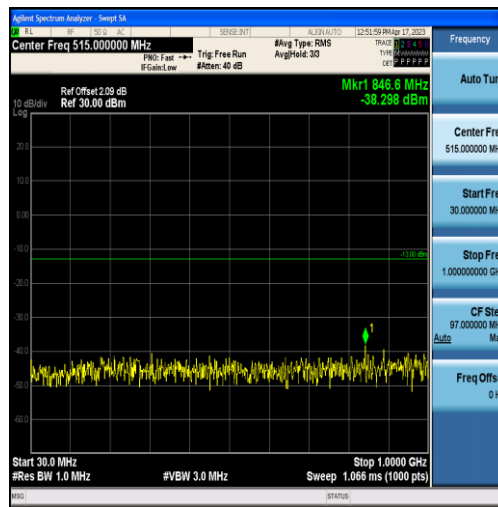
Band2-20MHz-16QAM-18900-100RB#0-Range1:30~1000MHz
