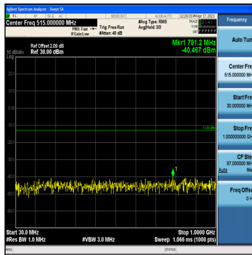
Band2-10MHz-16QAM-18900-50RB#0-Range1:30~1000MHz
