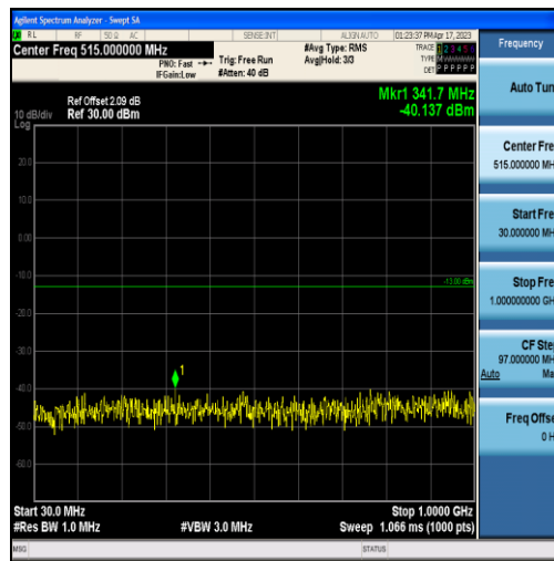
Band4-5MHz-16QAM-20175-25RB#0-Range1:30~1000MHz
