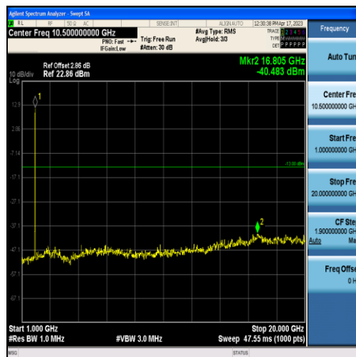
Band2-10MHz-16QAM-19150-50RB#0-Range2:1000~20000MHz
