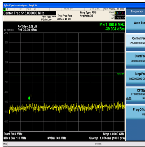
Band4-5MHz-QPSK-19975-25RB#0-Range1:30~1000MHz
