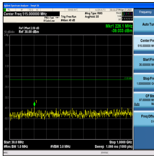
Band4-3MHz-16QAM-20175-15RB#0-Range1:30~1000MHz
