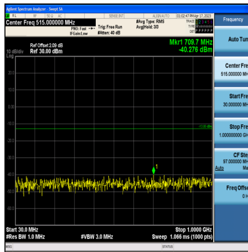
Band4-1.4MHz-16QAM-20175-6RB#0-Range1:30~1000MHz
