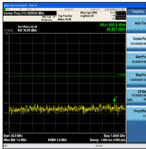
Band2-10MHz-QPSK-18650-50RB#0-Range1:30~1000MHz
