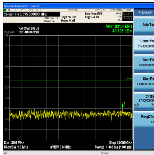
Band2-5MHz-QPSK-19175-25RB#0-Range1:30~1000MHz
