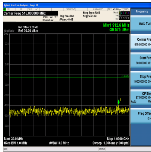
Band4-3MHz-16QAM-20385-15RB#0-Range1:30~1000MHz
