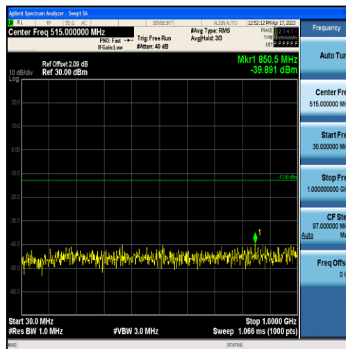
Band2-20MHz-QPSK-19100-100RB#0-Range1:30~1000MHz
