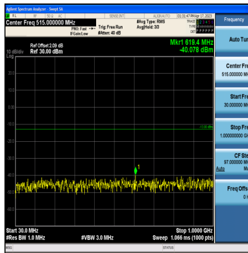
Band4-10MHz-16QAM-20175-50RB#0-Range1:30~1000MHz
