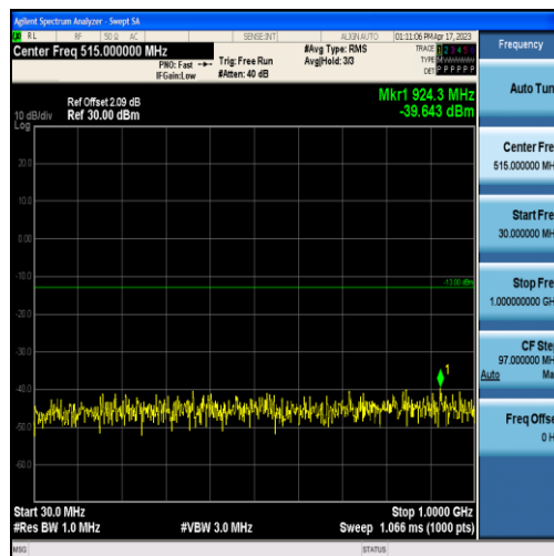
Band4-3MHz-16QAM-19965-15RB#0-Range1:30~1000MHz
