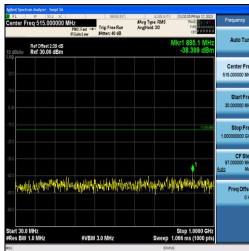
Band4-1.4MHz-16QAM-19957-6RB#0-Range1:30~1000MHz
