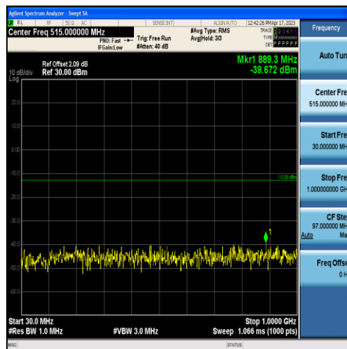
Band2-15MHz-QPSK-19125-75RB#0-Range1:30~1000MHz
