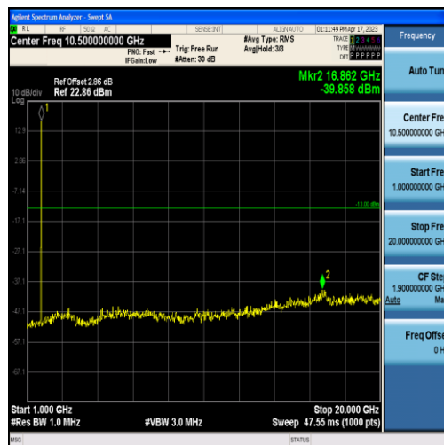
Band4-3MHz-16QAM-20385-15RB#0-Range2:1000~20000MHz
