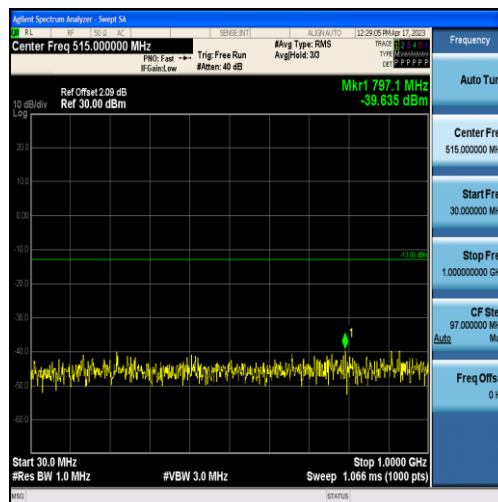
Band2-10MHz-16QAM-18650-50RB#0-Range1:30~1000MHz
