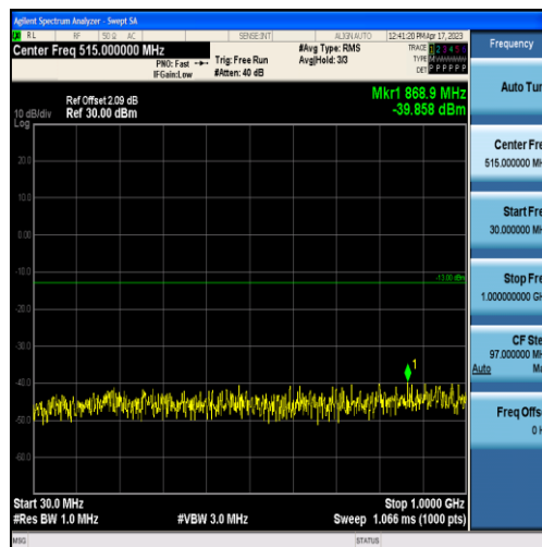
Band2-15MHz-16QAM-18675-75RB#0-Range1:30~1000MHz
