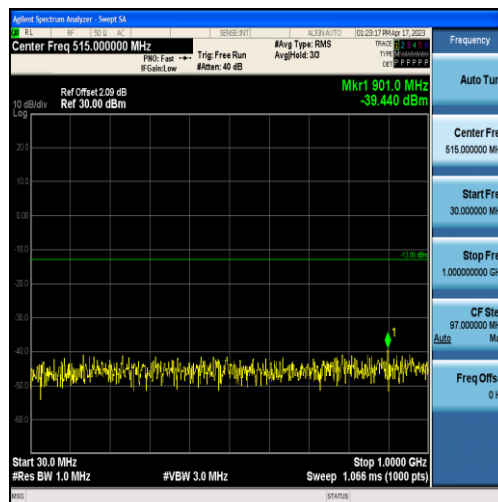
Band4-5MHz-16QAM-19975-25RB#0-Range1:30~1000MHz
