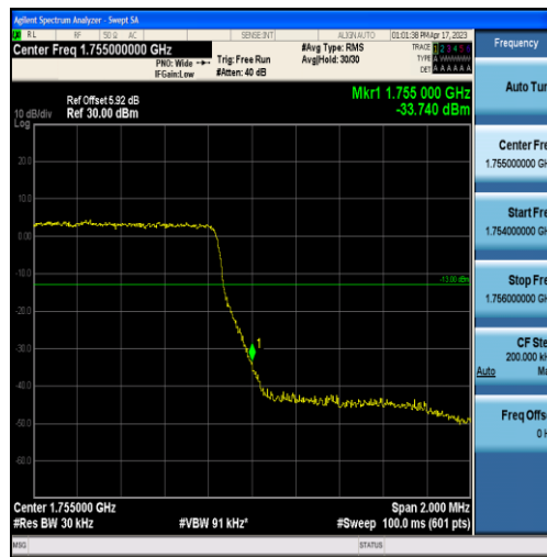
Band4-1.4MHz-QPSK-20393-6RB#0
