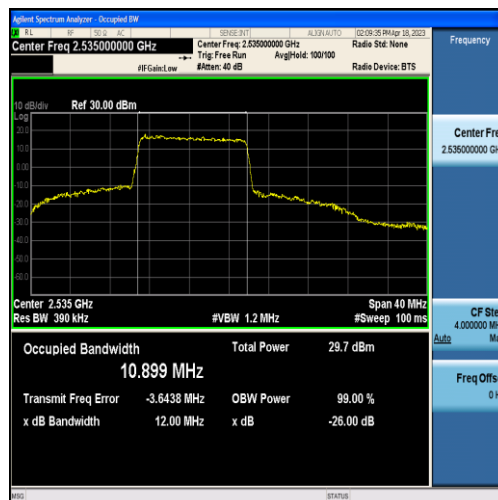
Band7-20MHz-QPSK-21100-60RB#0-10.899
