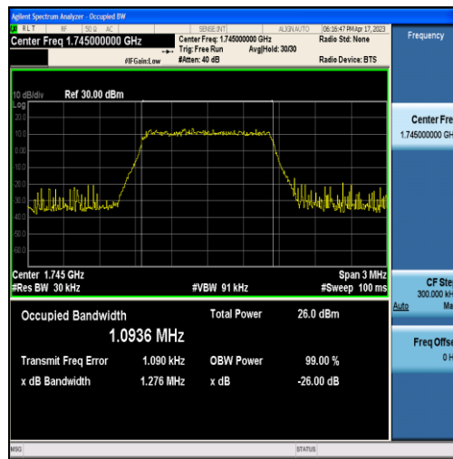
Band66-1.4MHz-16QAM-132322-6RB#0-1.0936
