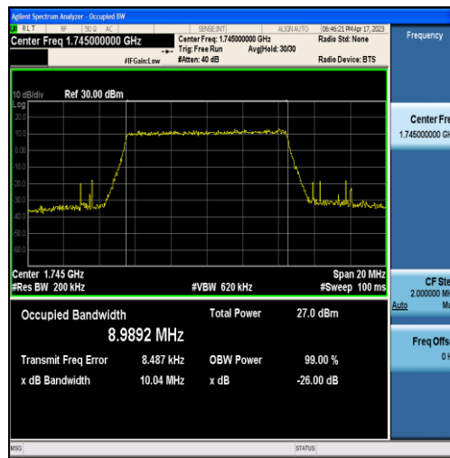
Band66-10MHz-16QAM-132322-50RB#0-8.9892
