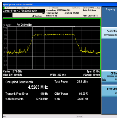
Band66-5MHz-16QAM-132647-25RB#0-4.5263
