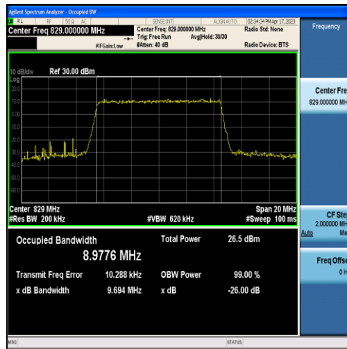
Band5-10MHz-16QAM-20450-50RB#0-8.9776
