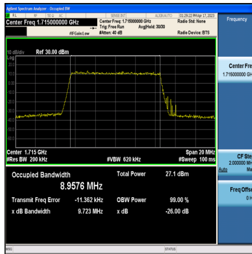
Band4-10MHz-16QAM-20000-50RB#0-8.9576
