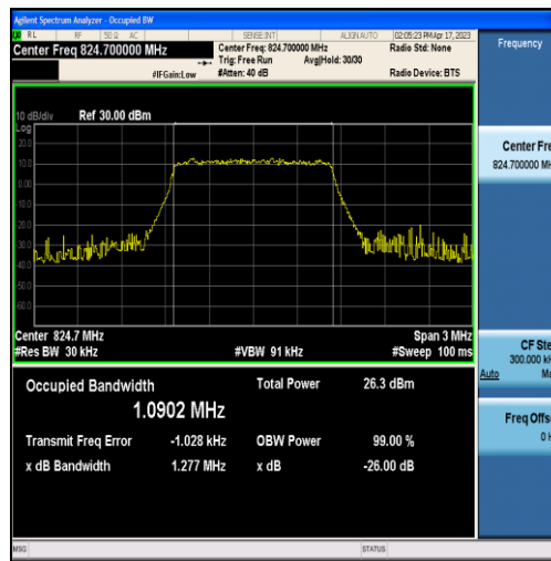
Band5-1.4MHz-QPSK-20407-6RB#0-1.0902
