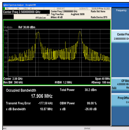
Band7-20MHz-16QAM-21350-60RB#0-17.906
