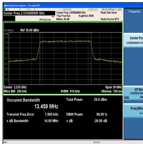
Band7-15MHz-QPSK-21100-75RB#0-13.459
