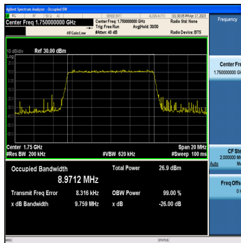
Band4-10MHz-16QAM-20350-50RB#0-8.9712
