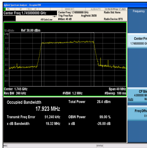
Band4-20MHz-QPSK-20300-100RB#0-17.923
