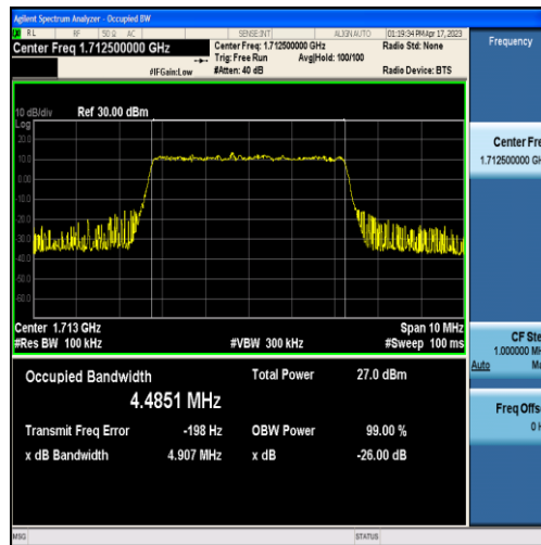
Band4-5MHz-16QAM-19975-25RB#0-4.4851
