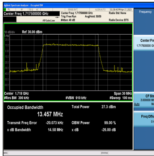
Band4-15MHz-16QAM-20025-75RB#0-13.457
