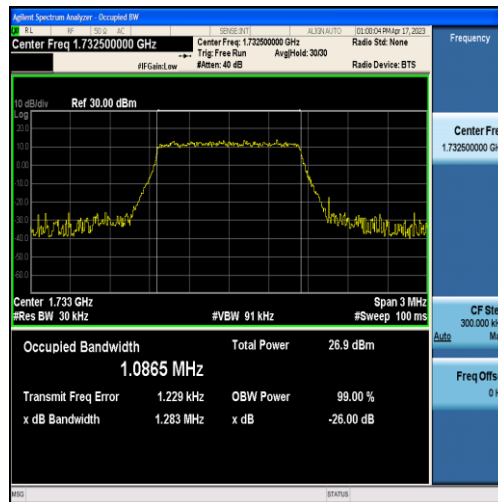
Band4-1.4MHz-QPSK-20175-6RB#0-1.0865
