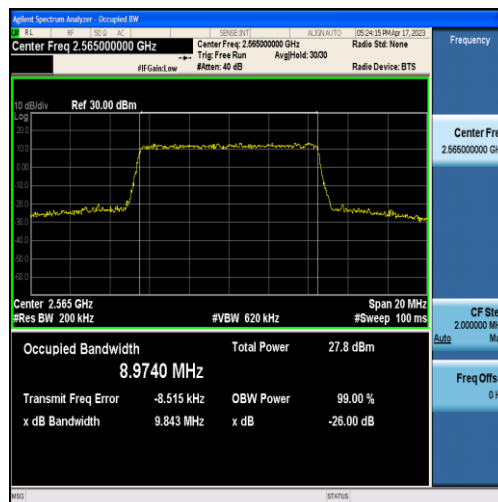
Band7-10MHz-16QAM-21400-50RB#0-8.9740
