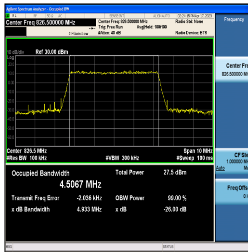
Band5-5MHz-QPSK-20425-25RB#0-4.5067
