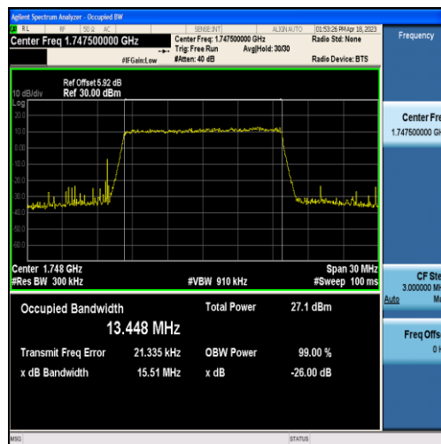
Band4-15MHz-16QAM-20325-75RB#0-13.448
