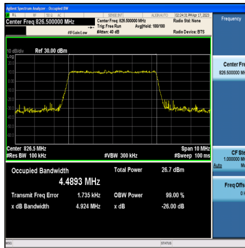
Band5-5MHz-16QAM-20425-25RB#0-4.4893
