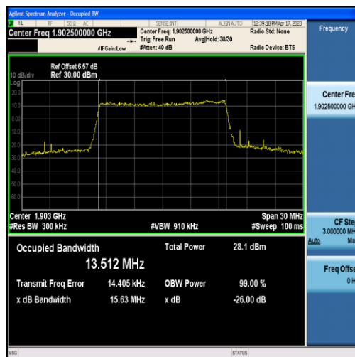
Band2-15MHz-16QAM-19125-75RB#0-13.512
