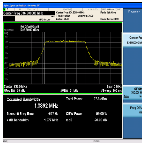
Band5-1.4MHz-QPSK-20525-6RB#0-1.0892
