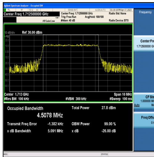
Band4-5MHz-QPSK-19975-25RB#0-4.5078
