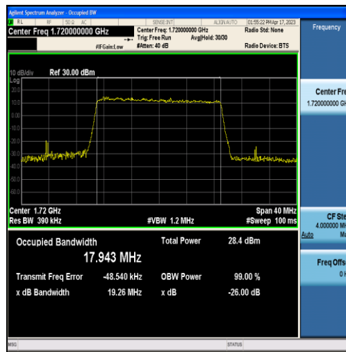
Band4-20MHz-QPSK-20050-100RB#0-17.943
