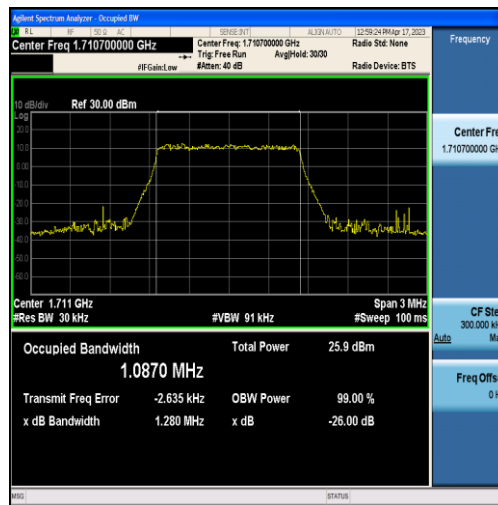
Band4-1.4MHz-16QAM-19957-6RB#0-1.0870
