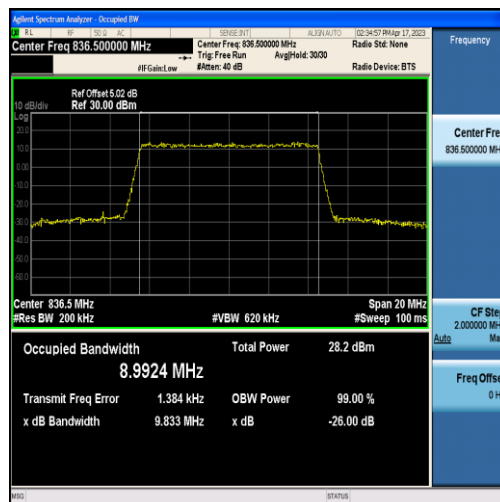
Band5-10MHz-QPSK-20525-50RB#0-8.9924
