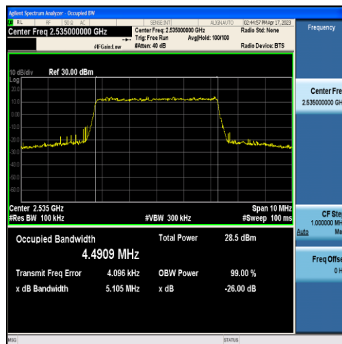
Band7-5MHz-QPSK-21100-25RB#0-4.4909
