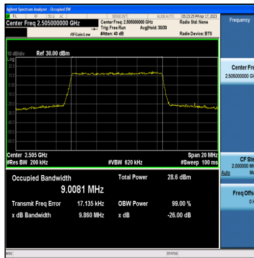
Band7-10MHz-QPSK-20800-50RB#0-9.0081
