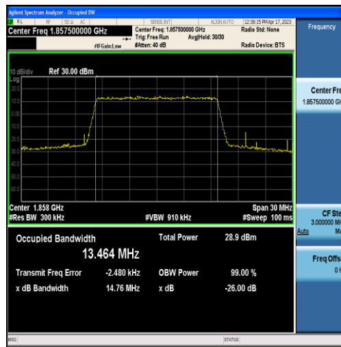
Band2-15MHz-QPSK-18675-75RB#0-13.464
