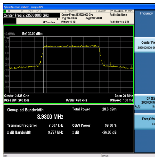
Band7-10MHz-QPSK-21100-50RB#0-8.9800
