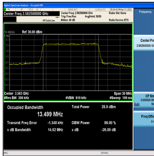
Band7-15MHz-QPSK-21375-75RB#0-13.499
