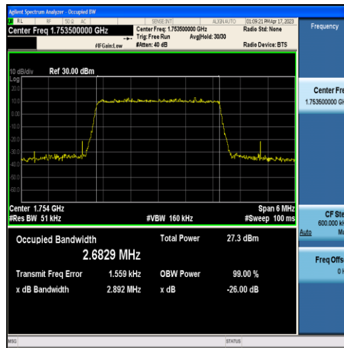
Band4-3MHz-QPSK-20385-15RB#0-2.6829
