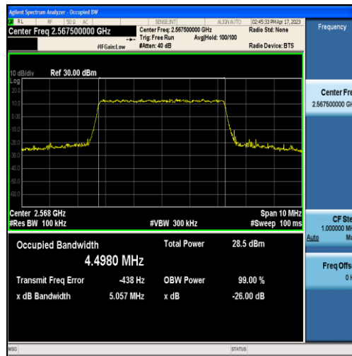
Band7-5MHz-QPSK-21425-25RB#0-4.4980
