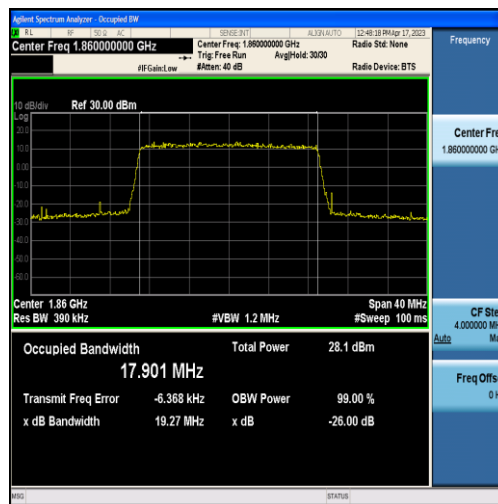
Band2-20MHz-16QAM-18700-100RB#0-17.901
