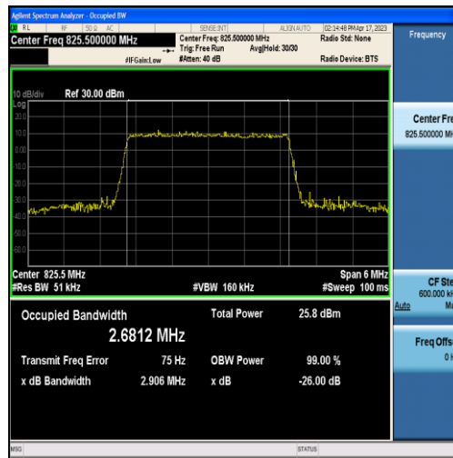
Band5-3MHz-16QAM-20415-15RB#0-2.6812
