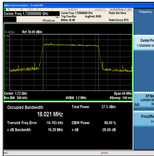
Band4-20MHz-16QAM-20050-100RB#0-18.021
