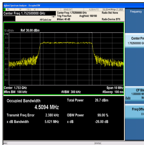
Band4-5MHz-16QAM-20375-25RB#0-4.5094
