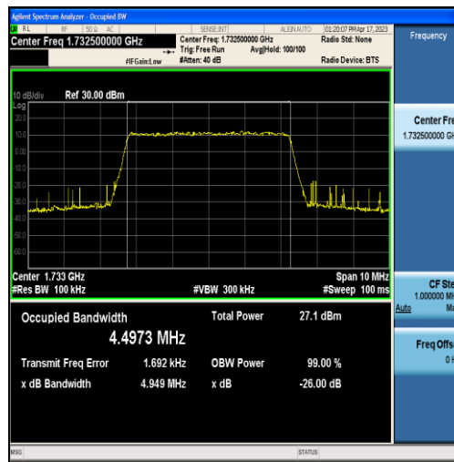
Band4-5MHz-16QAM-20175-25RB#0-4.4973
