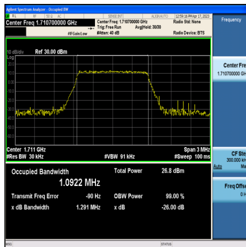
Band4-1.4MHz-QPSK-19957-6RB#0-1.0922
