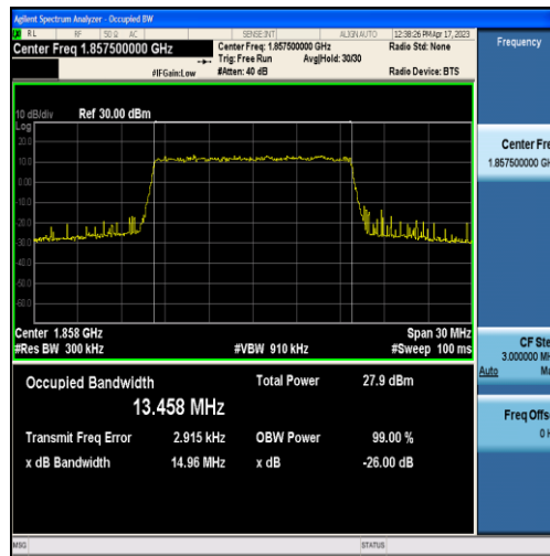
Band2-15MHz-16QAM-18675-75RB#0-13.458
