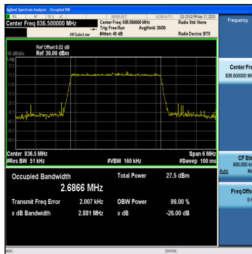
Band5-3MHz-QPSK-20525-15RB#0-2.6866
