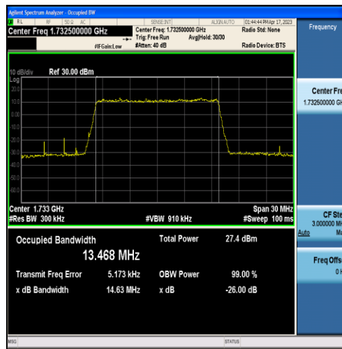
Band4-15MHz-16QAM-20175-75RB#0-13.468
