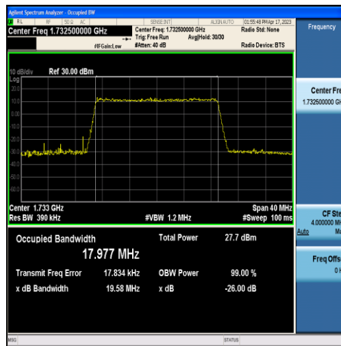
Band4-20MHz-16QAM-20175-100RB#0-17.977
