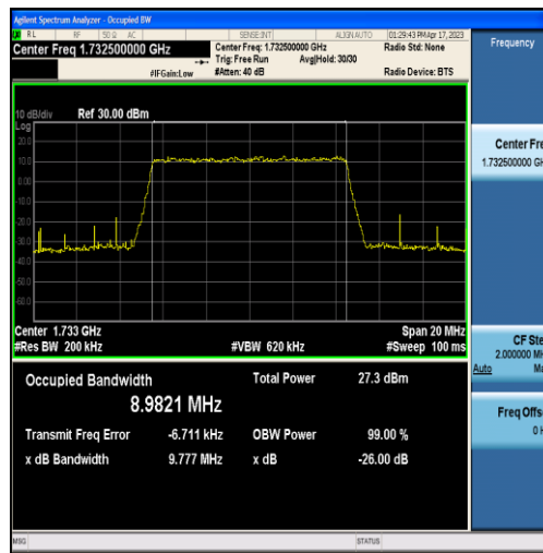
Band4-10MHz-16QAM-20175-50RB#0-8.9821
