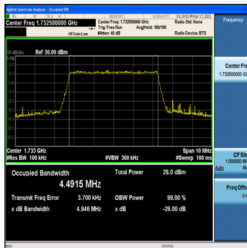
Band4-5MHz-QPSK-20175-25RB#0-4.4915
