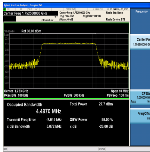
Band4-5MHz-QPSK-20375-25RB#0-4.4970
