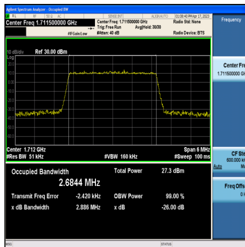
Band4-3MHz-QPSK-19965-15RB#0-2.6844
