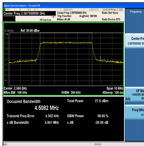
Band7-5MHz-16QAM-21425-25RB#0-4.5082
