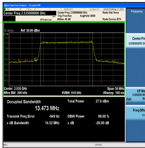
Band7-15MHz-16QAM-21100-75RB#0-13.473
