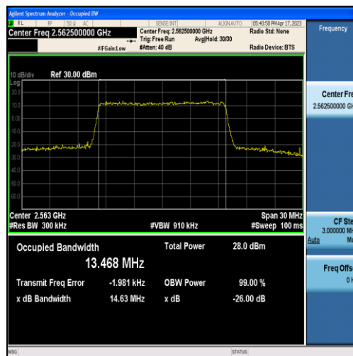
Band7-15MHz-16QAM-21375-75RB#0-13.468
