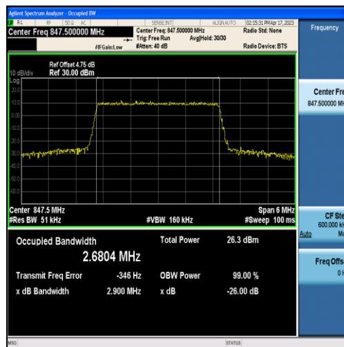
Band5-3MHz-16QAM-20635-15RB#0-2.6804
