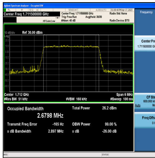
Band4-3MHz-16QAM-19965-15RB#0-2.6798
