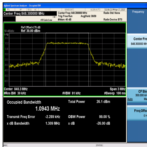
Band5-1.4MHz-16QAM-20643-6RB#0-1.0943
