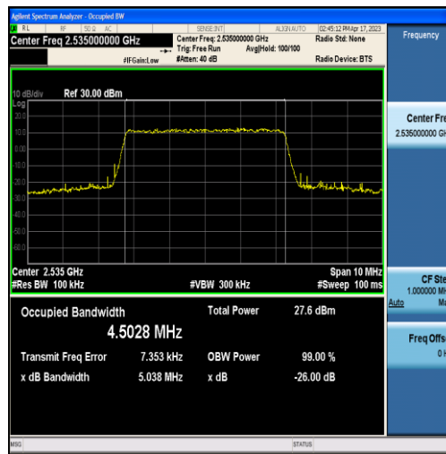
Band7-5MHz-16QAM-21100-25RB#0-4.5028
