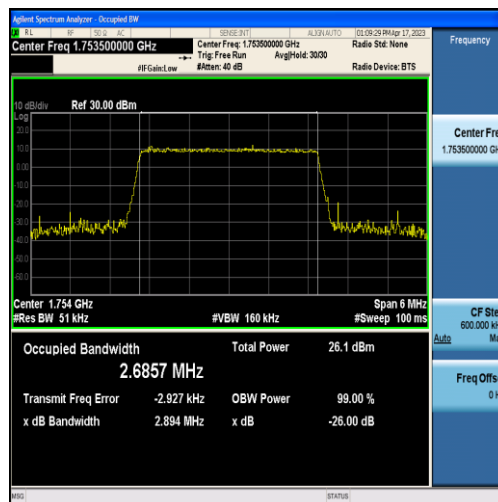
Band4-3MHz-16QAM-20385-15RB#0-2.6857
