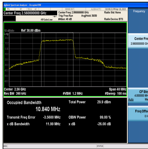
Band7-20MHz-QPSK-21350-60RB#0-10.840
