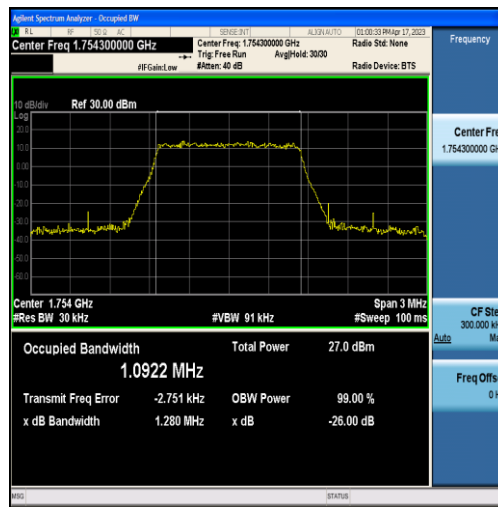
Band4-1.4MHz-QPSK-20393-6RB#0-1.0922
