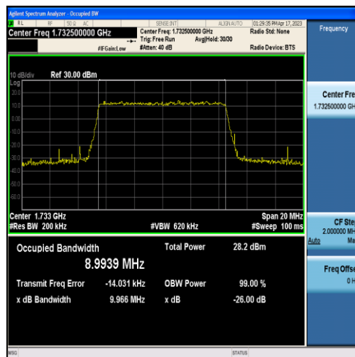
Band4-10MHz-QPSK-20175-50RB#0-8.9939
