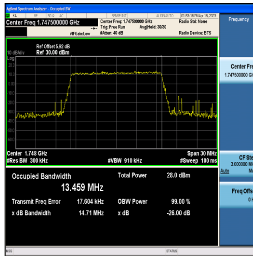
Band4-15MHz-QPSK-20325-75RB#0-13.459
