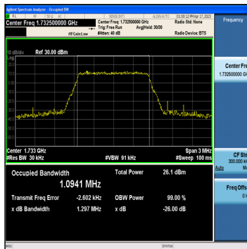
Band4-1.4MHz-16QAM-20175-6RB#0-1.0941
