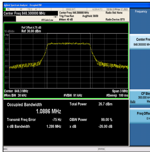
Band5-1.4MHz-QPSK-20643-6RB#0-1.0886
