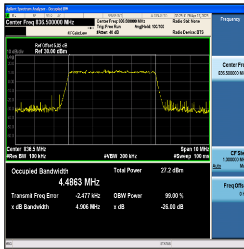
Band5-5MHz-16QAM-20525-25RB#0-4.4863
