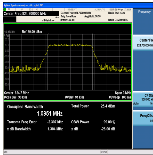
Band5-1.4MHz-16QAM-20407-6RB#0-1.0951
