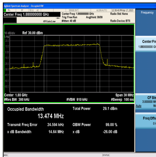
Band2-15MHz-QPSK-18900-75RB#0-13.474
