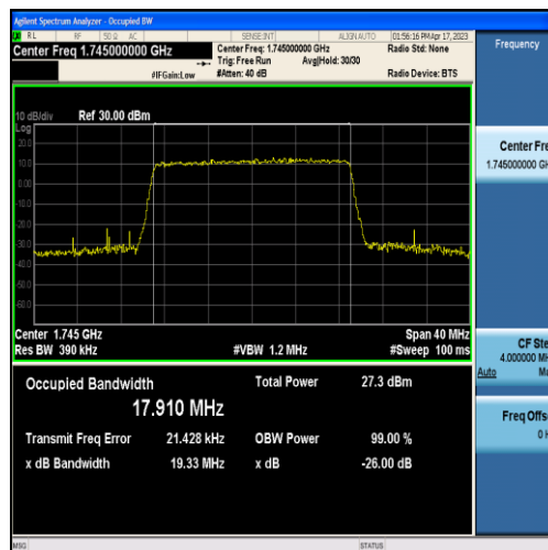
Band4-20MHz-16QAM-20300-100RB#0-17.910
