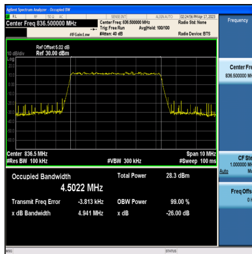
Band5-5MHz-QPSK-20525-25RB#0-4.5022
