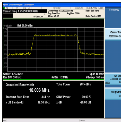
Band4-20MHz-QPSK-20175-100RB#0-18.006
