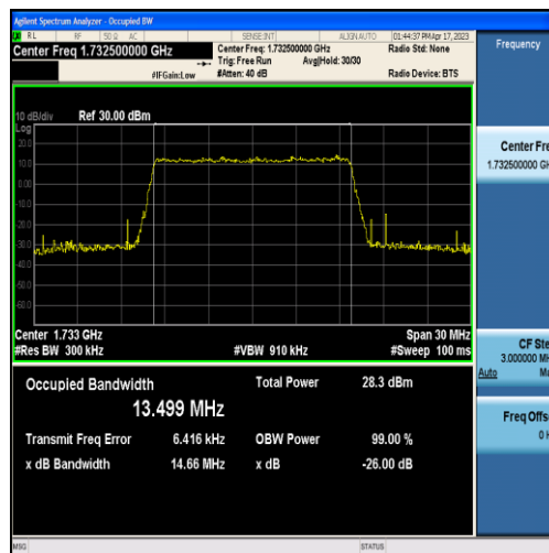
Band4-15MHz-QPSK-20175-75RB#0-13.499
