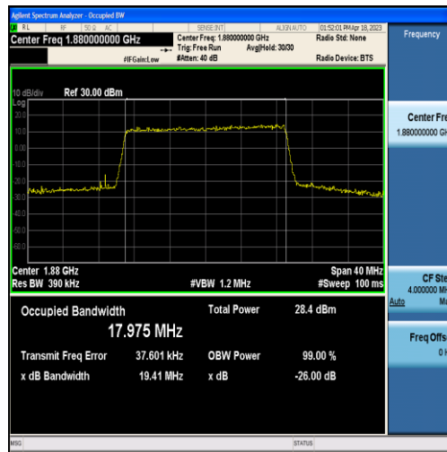
Band2-20MHz-16QAM-18900-100RB#0-17.975
