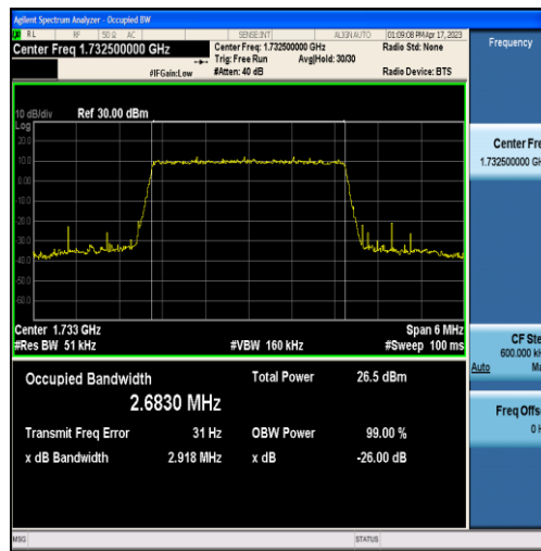
Band4-3MHz-16QAM-20175-15RB#0-2.6830
