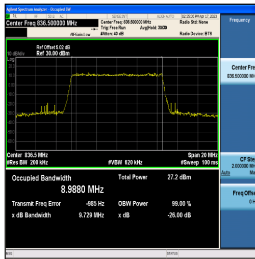
Band5-10MHz-16QAM-20525-50RB#0-8.9880
