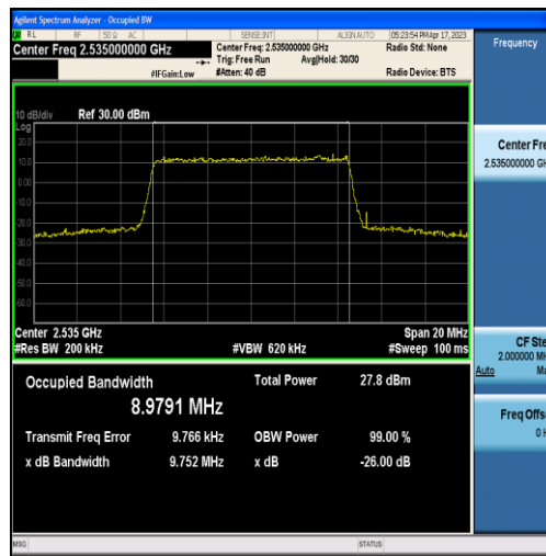
Band7-10MHz-16QAM-21100-50RB#0-8.9791
