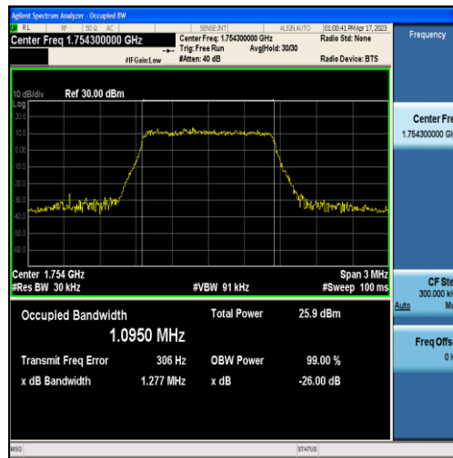
Band4-1.4MHz-16QAM-20393-6RB#0-1.0950
