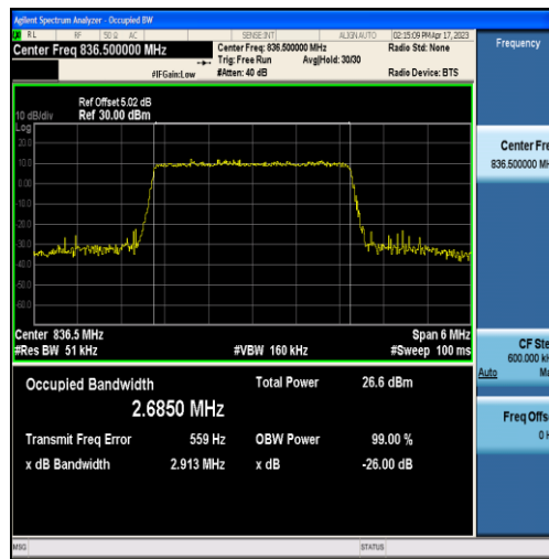
Band5-3MHz-16QAM-20525-15RB#0-2.6850
