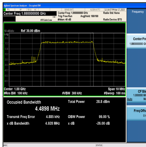
Band2-5MHz-QPSK-18900-25RB#0-4.4898
