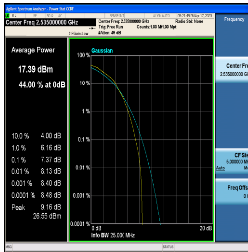
Band7-5MHz-16QAM-21100-25RB#0
