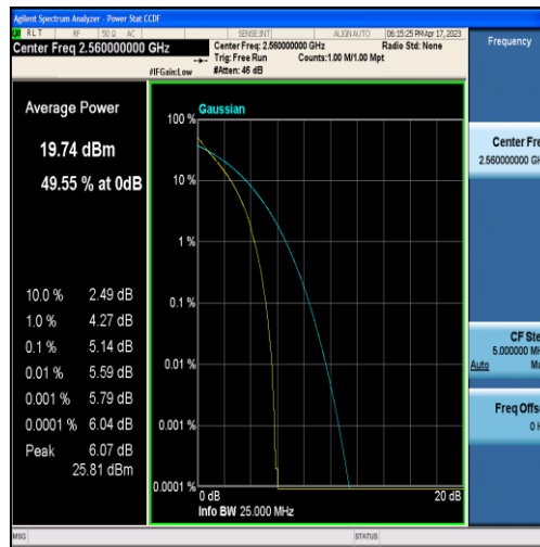
Band7-20MHz-QPSK-21350-60RB#0
