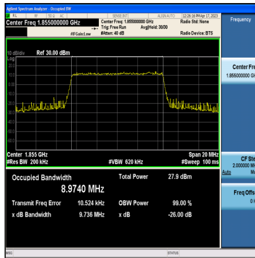
Band2-10MHz-16QAM-18650-50RB#0-8.9740
