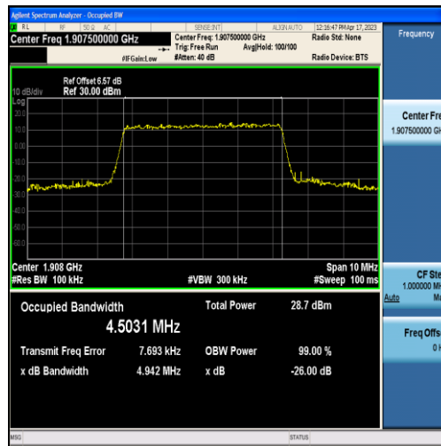
Band2-5MHz-QPSK-19175-25RB#0-4.5031
