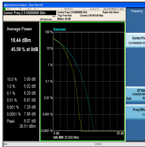
Band7-20MHz-16QAM-20850-60RB#0
