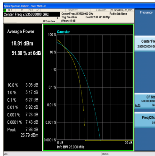
Band7-20MHz-QPSK-21100-60RB#0
