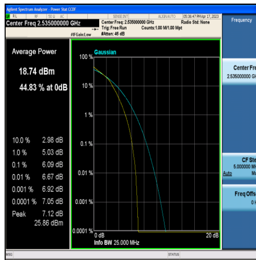
Band7-10MHz-16QAM-21100-50RB#0
