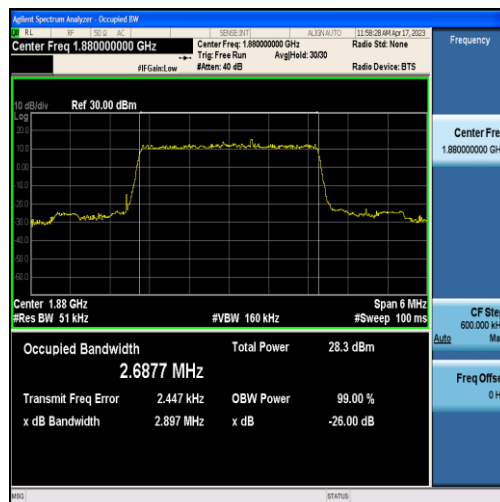
Band2-3MHz-QPSK-18900-15RB#0-2.6877
