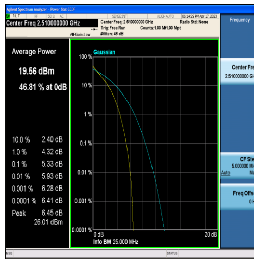
Band7-20MHz-QPSK-20850-60RB#0
