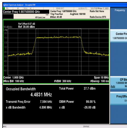
Band2-5MHz-16QAM-19175-25RB#0-4.4831
