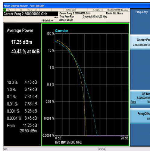
Band7-20MHz-16QAM-21350-60RB#0
