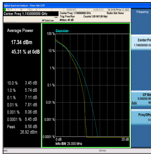
Band66-3MHz-16QAM-132322-15RB#0
