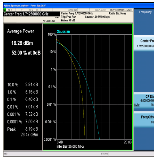
Band66-5MHz-QPSK-131997-25RB#0
