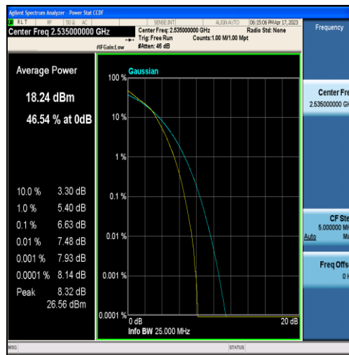
Band7-20MHz-16QAM-21100-60RB#0
