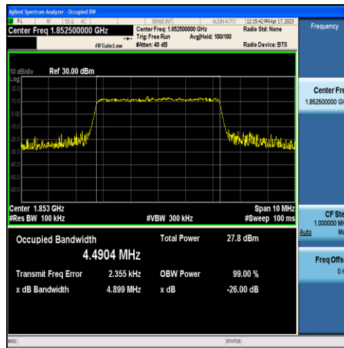
Band2-5MHz-16QAM-18625-25RB#0-4.4904
