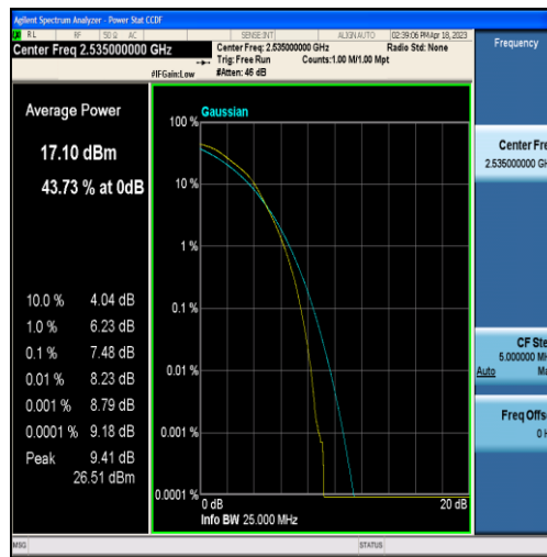
Band7-20MHz-16QAM-21100-100RB#0
