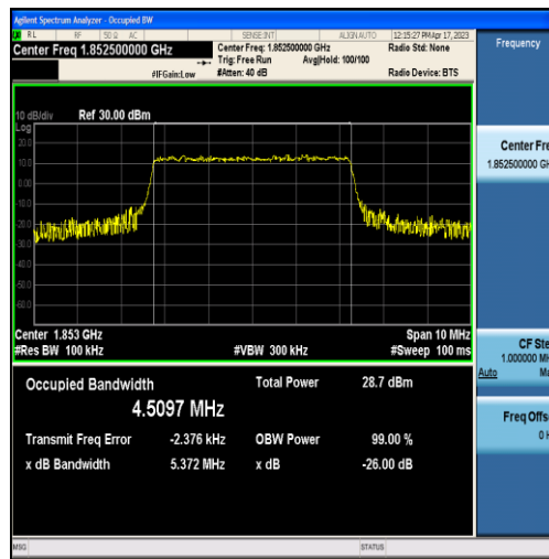
Band2-5MHz-QPSK-18625-25RB#0-4.5097
