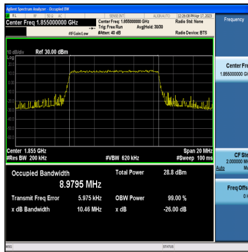
Band2-10MHz-QPSK-18650-50RB#0-8.9795
