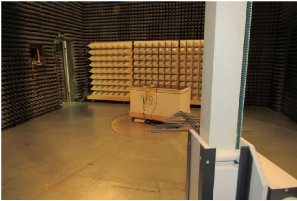
Test setup radiated between 0.2 to 1 GHz
