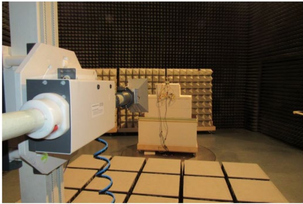
Test setup radiated above 1 GHz
