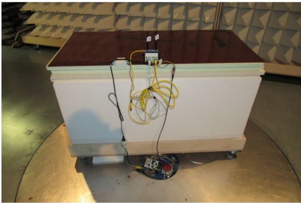
Test setup radiated EUT view below 1 GHz
