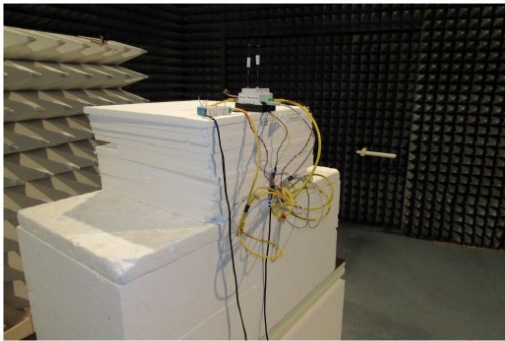
Test setup radiated EUT view above 1 GHz
