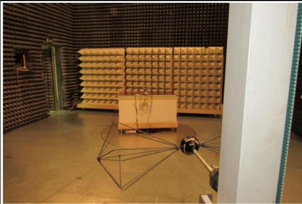
Test setup radiated below 0.2 GHz
