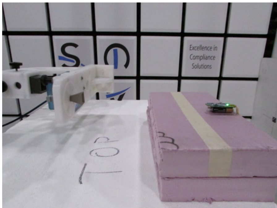
Figure 6: Radiated Emissions – Side – Above 18GHz
