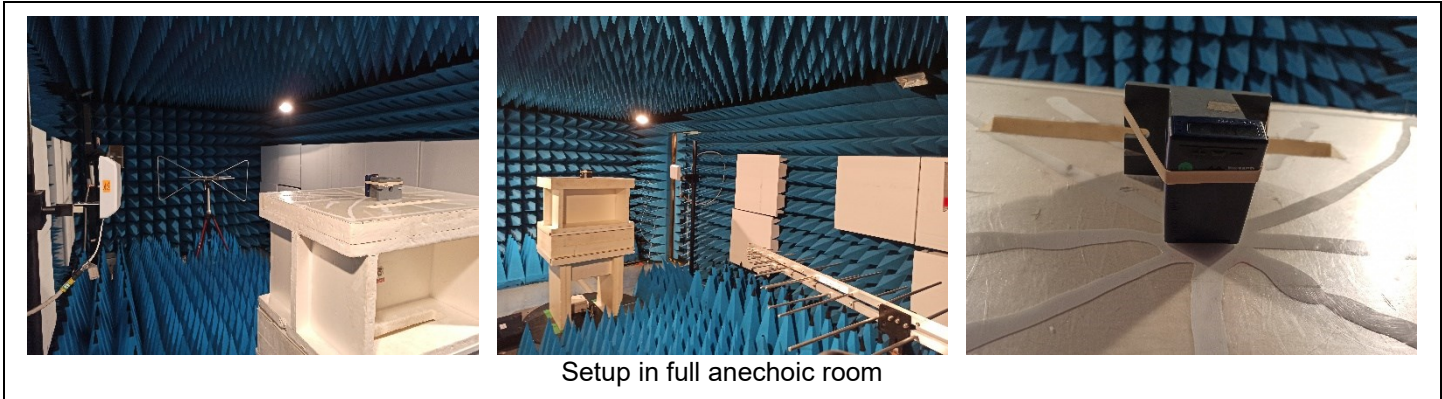
Photograph for Unwanted Emission in restricted frequency bands
