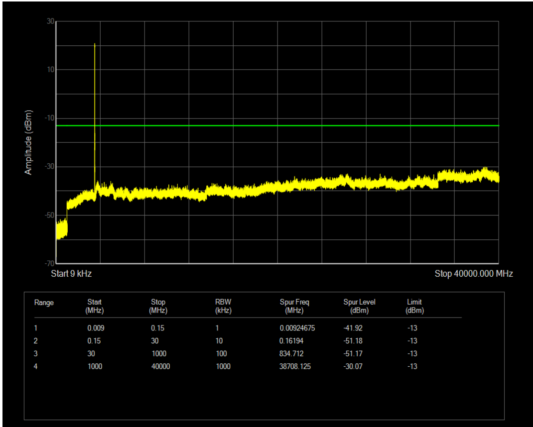
n77(3450-3550) SCS=30kHz DFT_QPSK BW=10MHz Channel=633334 RB=1@0
