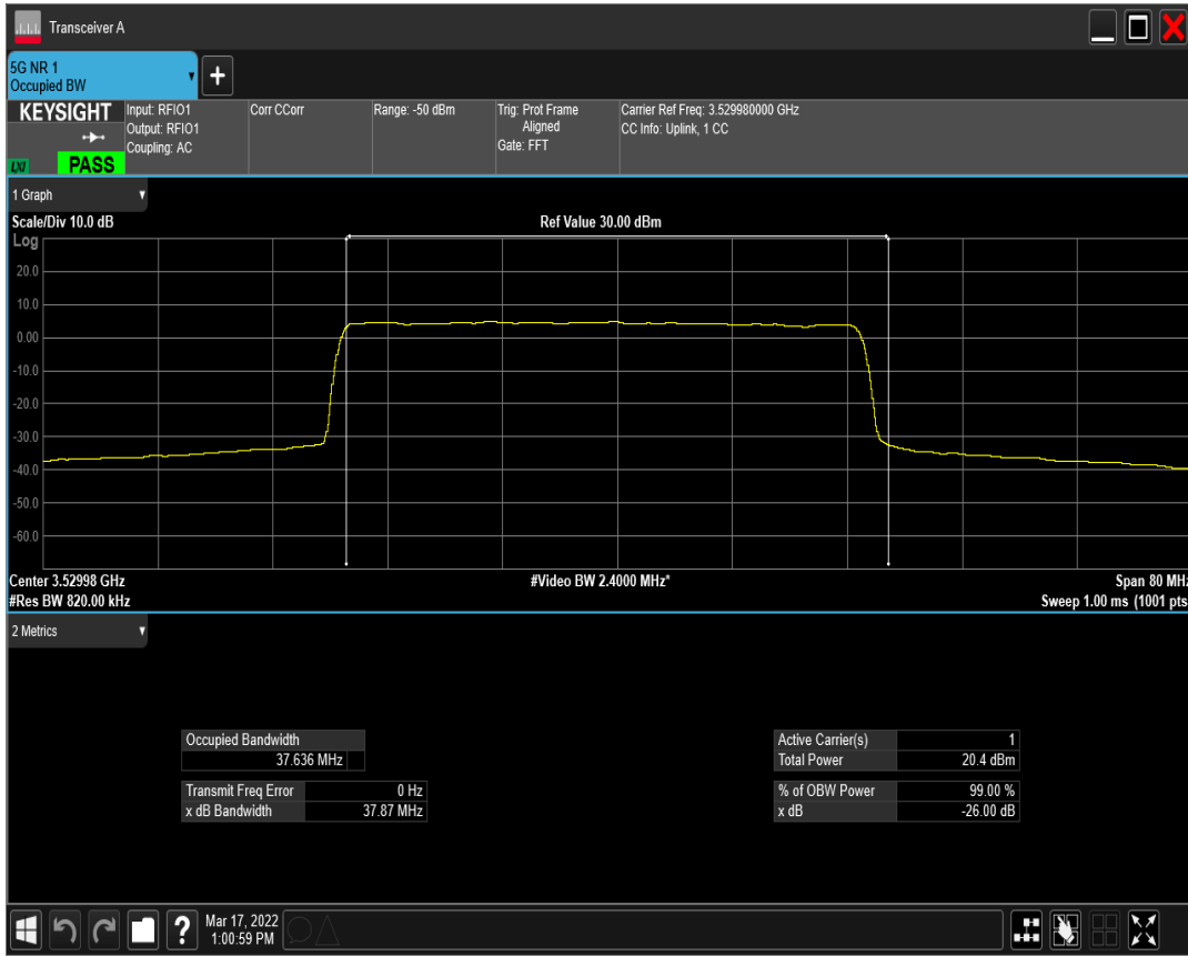
n77(3450-3550) SCS=30kHz CP_QPSK BW=40MHz Channel=635332 RB=106@0
