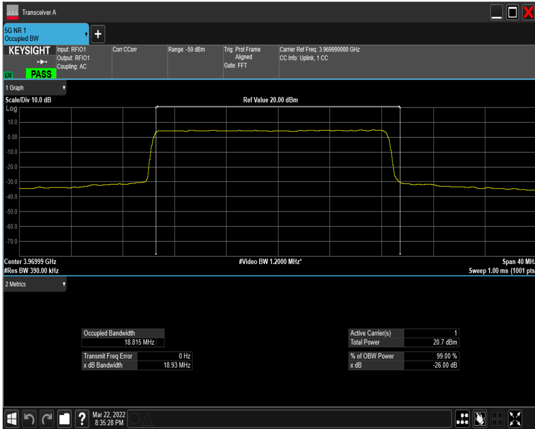
n77(3700-3980) SCS=15kHz DFT_QAM64 BW=20MHz Channel=664666 RB=100@0
