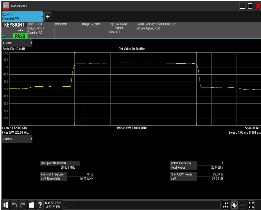
n77(3700-3980) SCS=15kHz DFT_QAM64 BW=40MHz Channel=648000 RB=216@0
