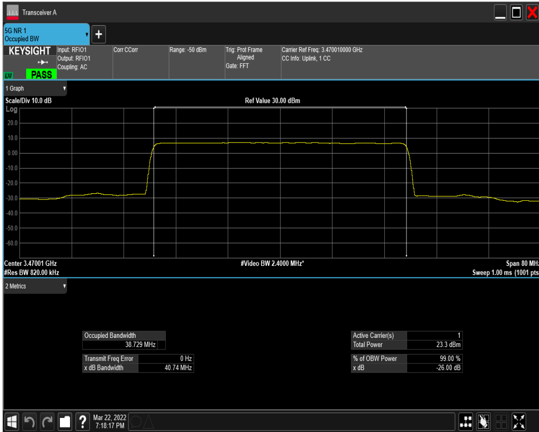
n77(3450-3550) SCS=15kHz DFT_QAM64 BW=40MHz Channel=631334 RB=216@0
