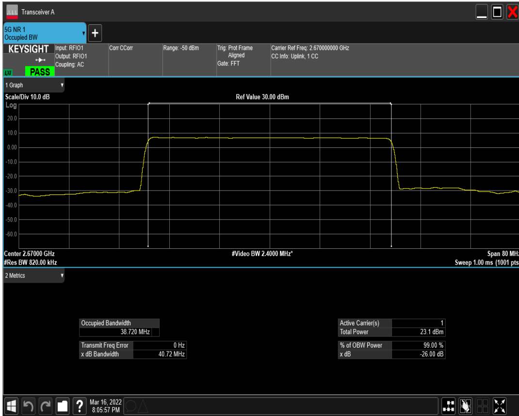
n41 SCS=15kHz DFT_QAM64 BW=40MHz Channel=534000 RB=216@0
