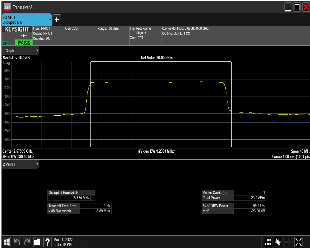
n41 SCS=15kHz DFT_QAM64 BW=20MHz Channel=535998 RB=100@0
