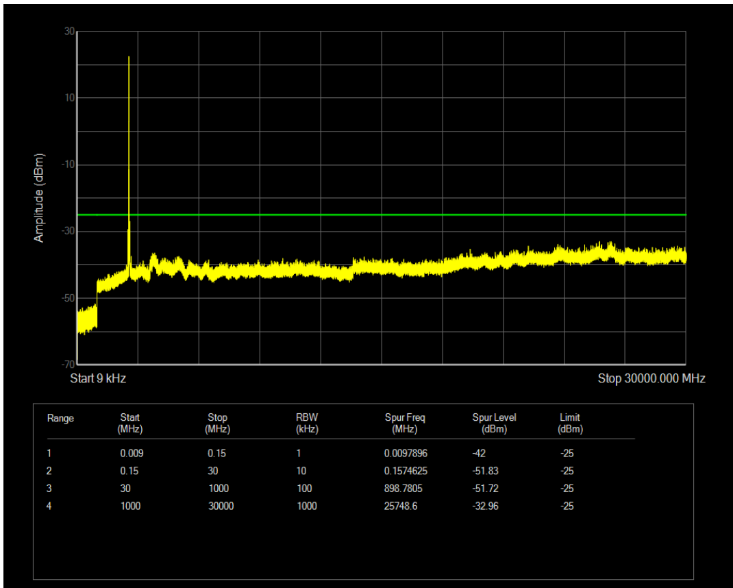
n41 SCS=15kHz DFT_QPSK BW=50MHz Channel=518601 RB=1@269
