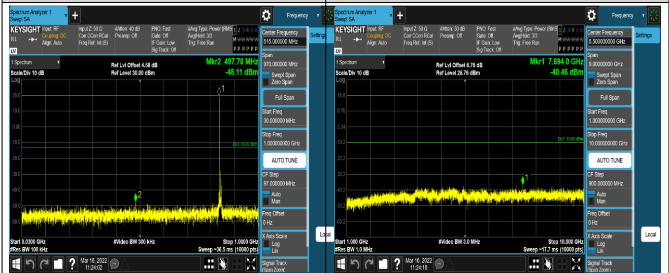
Band5-10MHz-16QAM-20600-1RB#0-Range1:30~1000MHz Band5-10MHz-16QAM-20600-1RB#0-Range2:1000~10000MHz
