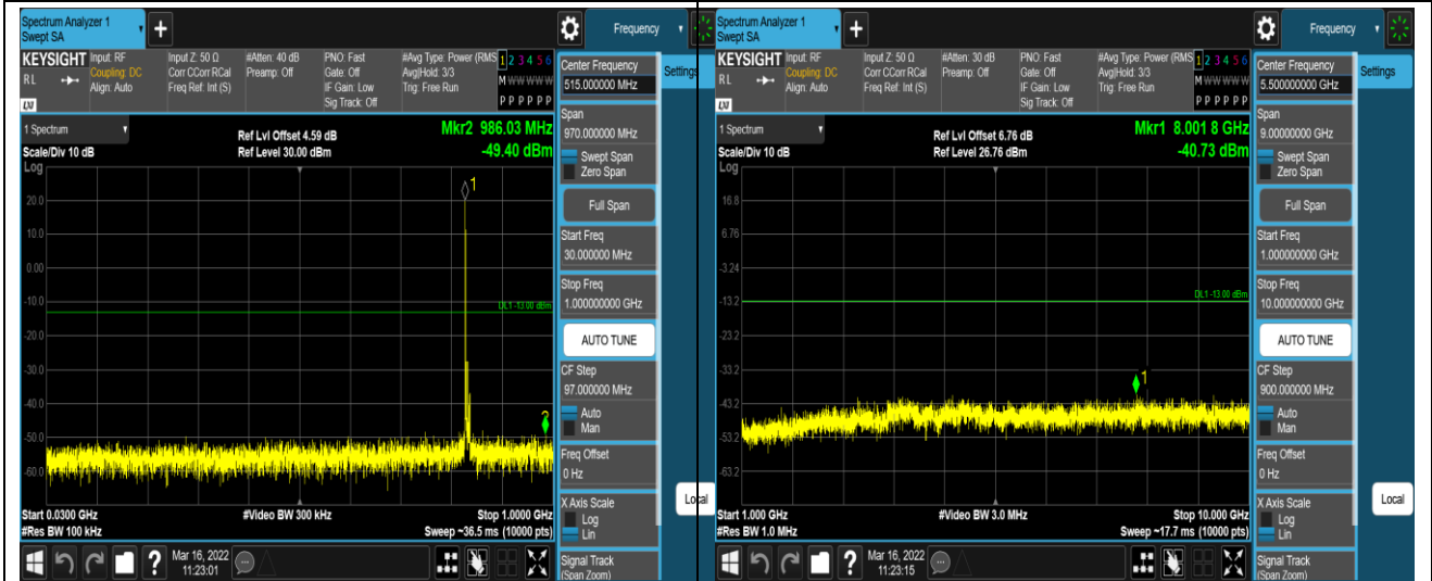
Band5-10MHz-16QAM-20600-1RB#0-Range1:30~1000MHz Band5-10MHz-16QAM-20600-1RB#0-Range2:1000~10000MHz
