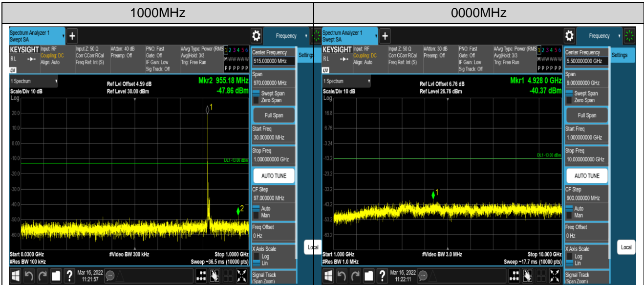
Band5-10MHz-16QAM-20525-1RB#0-Range1:30~1000MHz Band5-10MHz-16QAM-20525-1RB#0-Range2:1000~10000MHz
