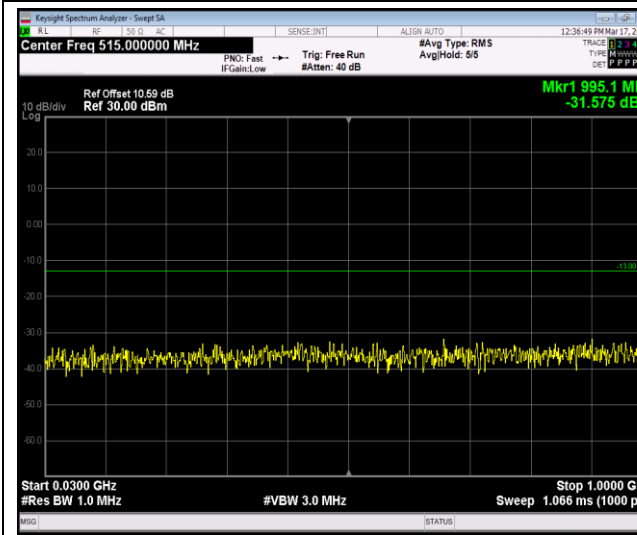
Band66-1.4MHz-16QAM-131979-1RB#0-Range1:30~1000MHz
