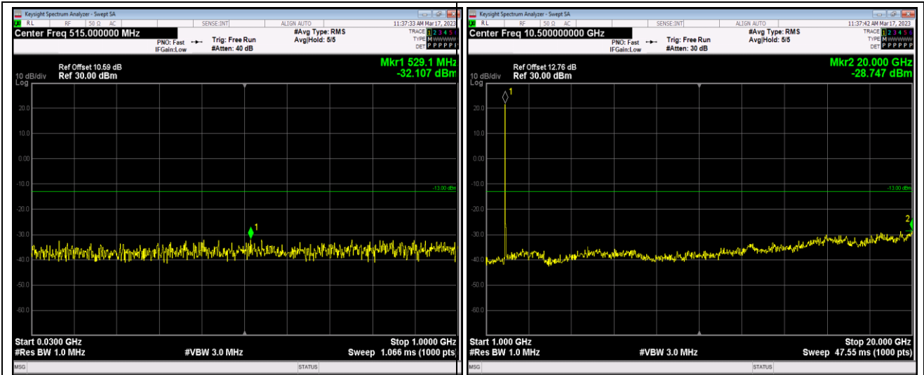
Band25-20MHz-16QAM-26365-1RB#0-Range1:30~1000MHz
