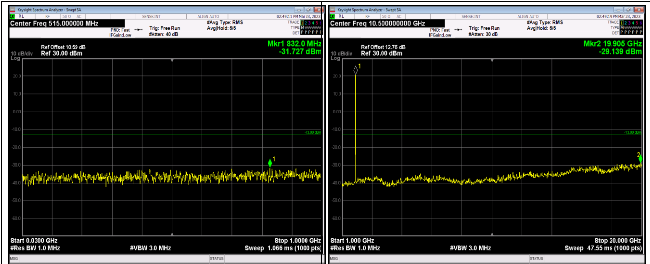
Band25-1.4MHz-64QAM-26683-1RB#0-Range1:30 ~1000MHz
