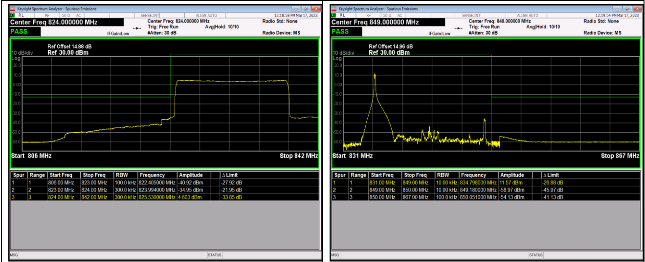
Band26-15MHz-QPSK-26965-1RB#74
