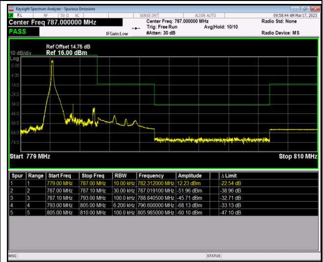
Band13-5MHz-QPSK-23255-25RB#0
