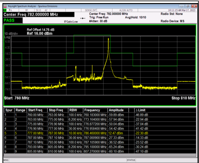
Band13-10MHz-16QAM-23230-1RB#0
