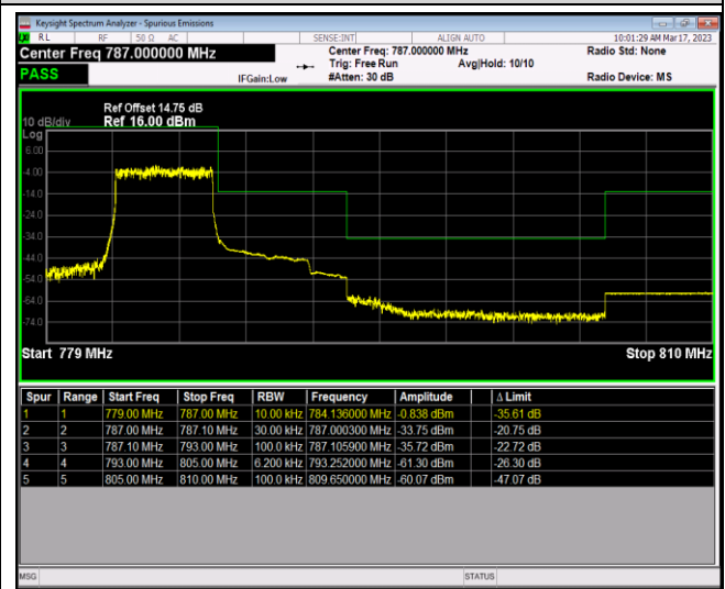
Band13-5MHz-16QAM-23205-1RB#24
