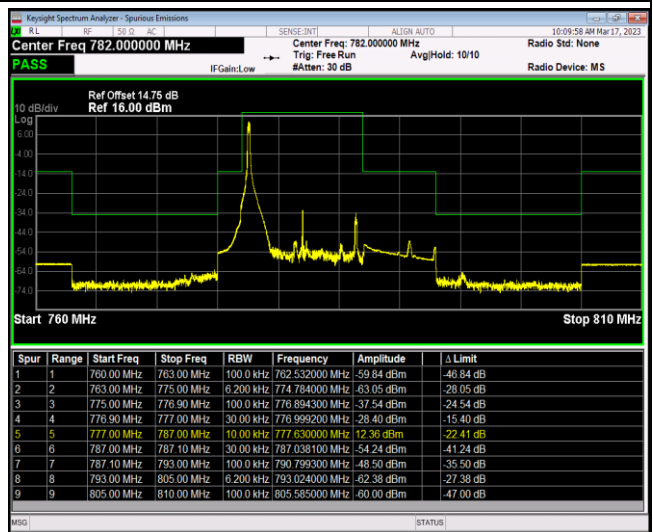
Band13-10MHz-16QAM-23230-50RB#0
