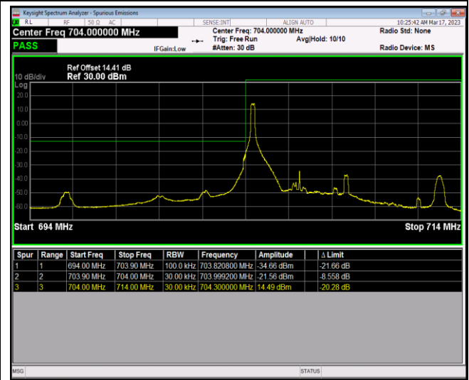
Band17-5MHz-QPSK-23755-25RB#0
