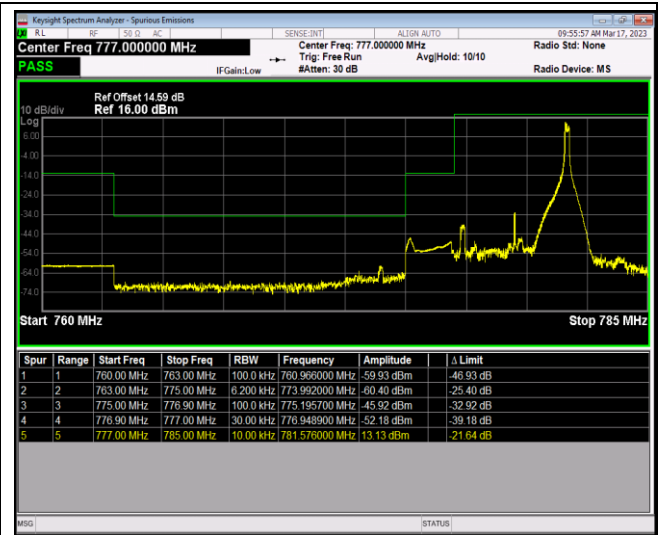
Band13-5MHz-QPSK-23255-1RB#0
