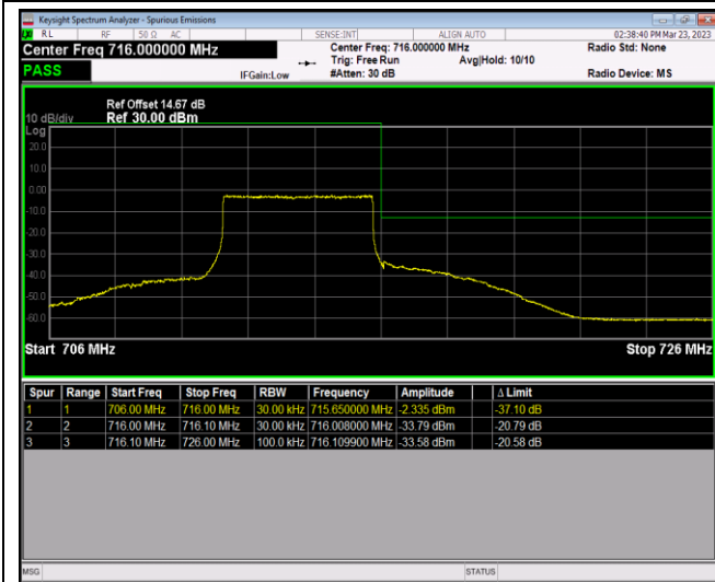
Band17-10MHz-QPSK-23780-1RB#49
