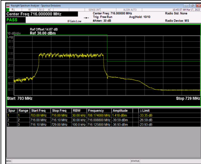
Band17-10MHz-64QAM-23780-1RB#49
