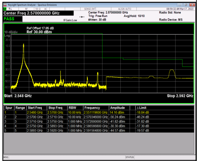
Band7-20MHz-QPSK-21350-100RB#0
