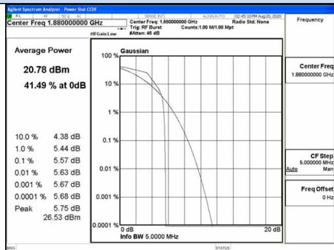
Channel 661/ 1880 MHz
