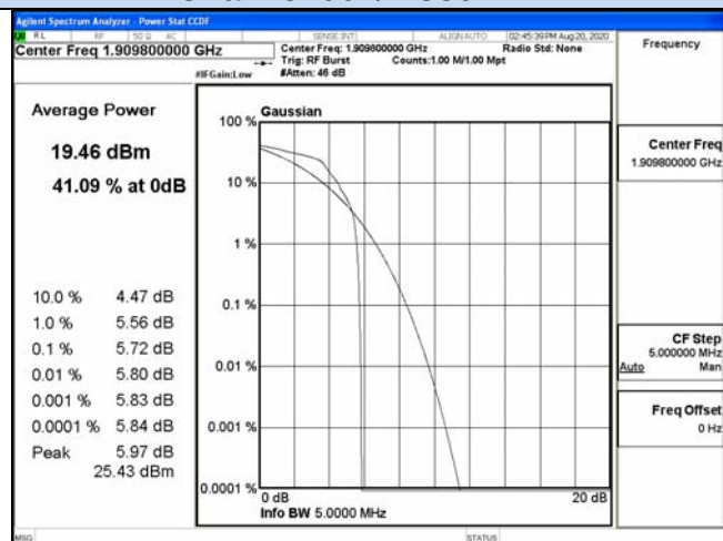
Channel 810/ 1909.8 MHz
