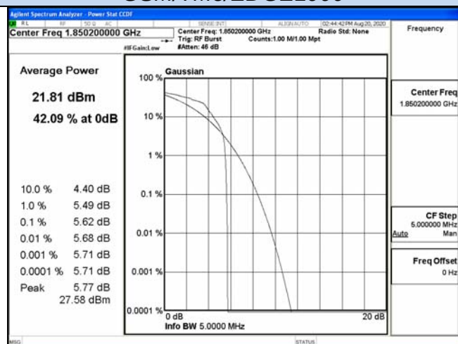
Channel 512/ 1850.2 MHz
