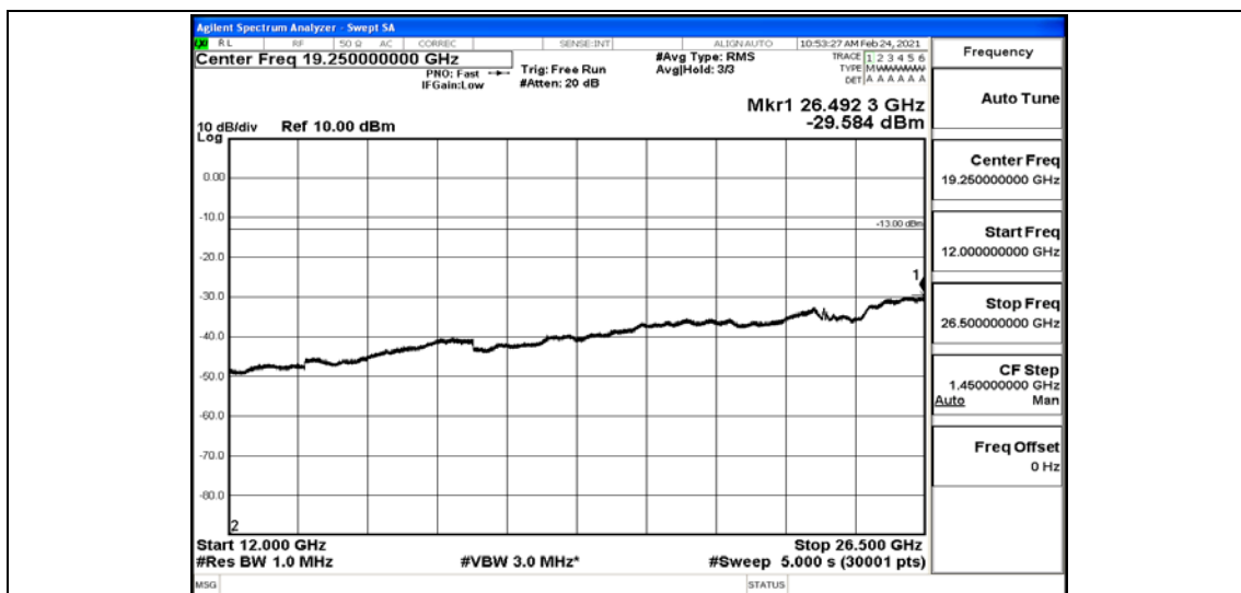
Band66-10MHz-QPSK-132022-1RB#0-Range1:0.009~0.15MHz
